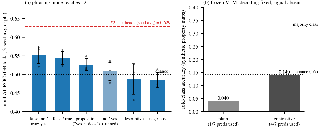
Figure 4: Controlled mechanism ablations. (a) Noul candidate phrasing on three seed-averaged stable checkpoints (same weights; only candidate text varies). No phrasing reaches the per-task-head reference (0.629, dashed); the best (“false: no / true: yes”, 0.553 \pm 0.023 ) beats the trained phrasing (hatched) on all three seeds — reversing the single-checkpoint finding, i.e., inference-level ablations are also checkpoint-dependent. (b) Frozen VLM on synthetic property maps (multimodal route-A pilot): plain candidate likelihood collapses to one class (acc 0.040, 1/7 classes used); contrastive decoding removes the collapse (0.140, 4/7) but remains at chance — decoding fixed, signal absent.
