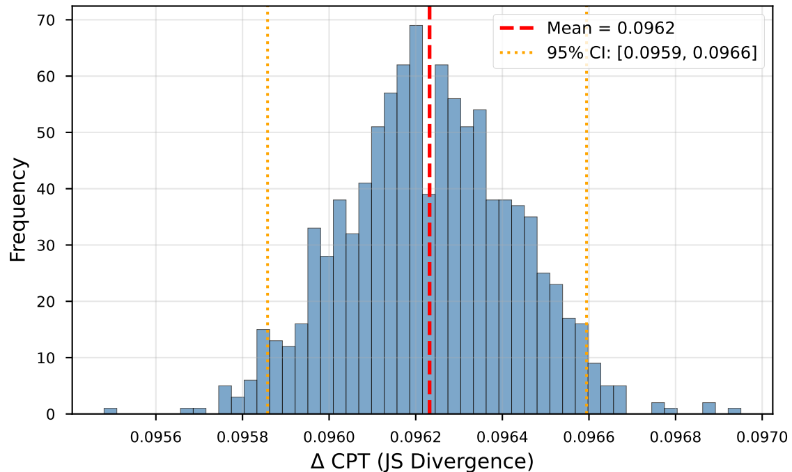
Bootstrap Distribution of CPT Contribution
