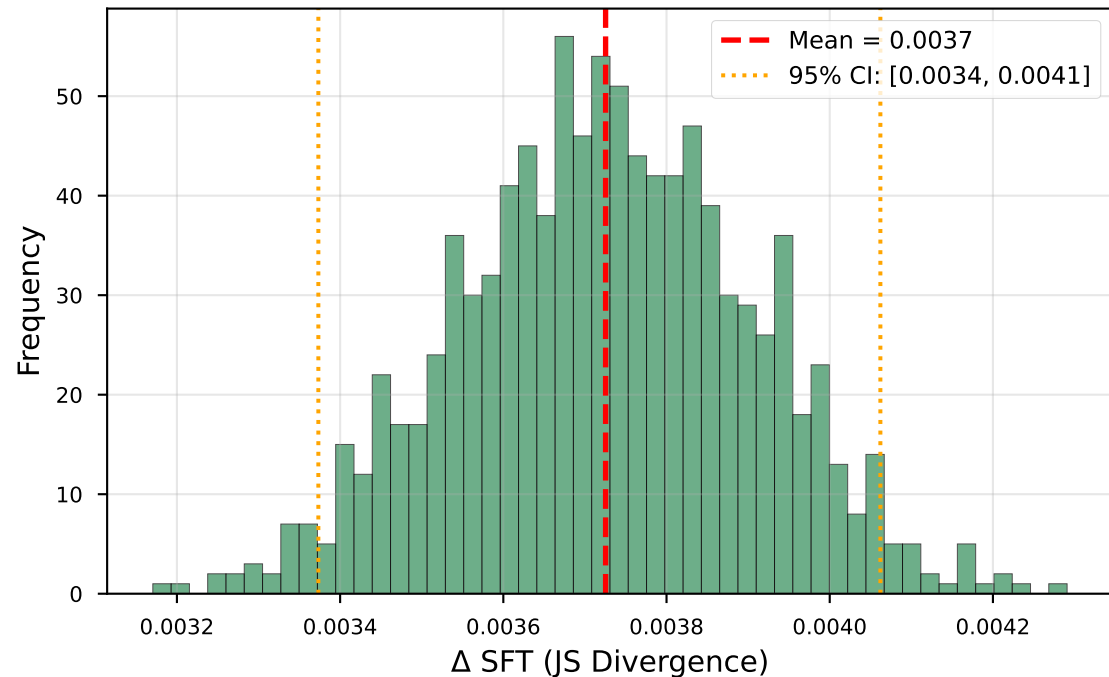
Bootstrap Distribution of SFT Contribution
