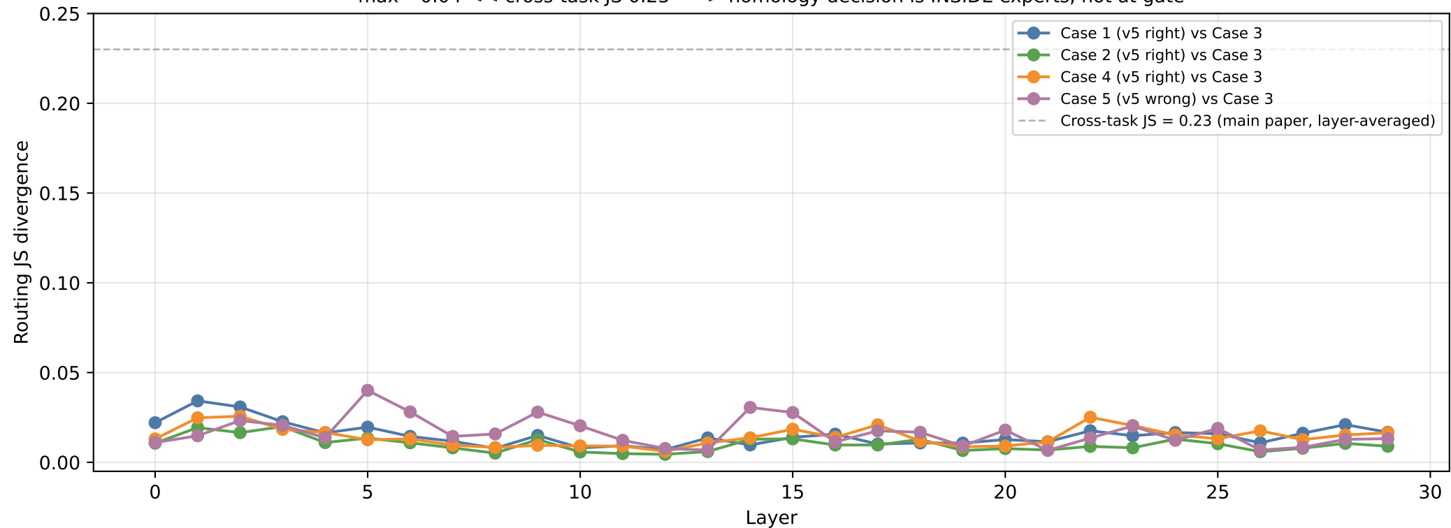
Per-layer routing JS divergence: homologous vs non-homologous case max \sim 0.04 \ll cross-task JS 0.23 \implies homology decision is INSIDE experts, not at gate
