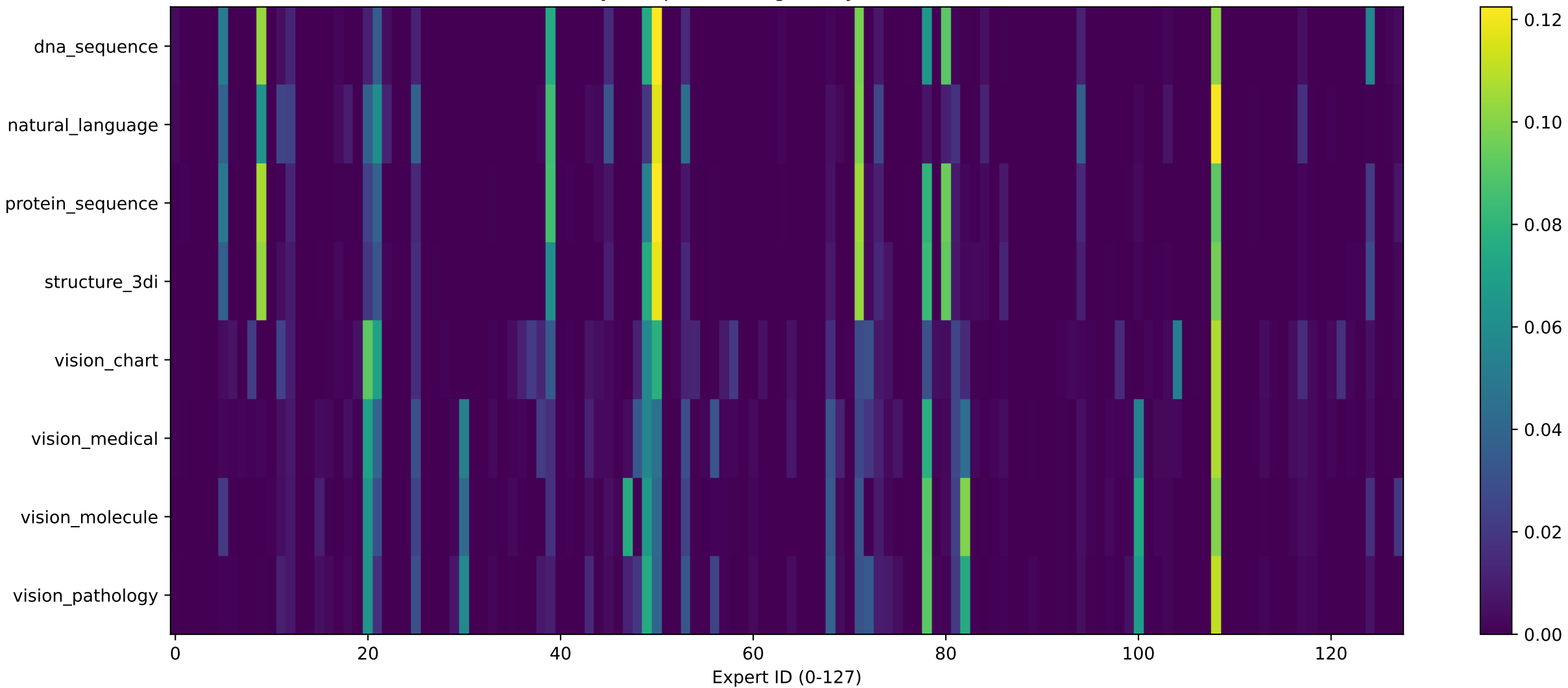
Modality x Expert routing at Layer 12 (normalized)
