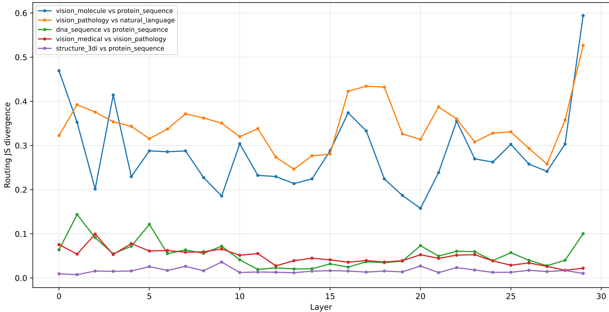
OmniGene-4-MM: per-layer routing JS (key modality pairs)
