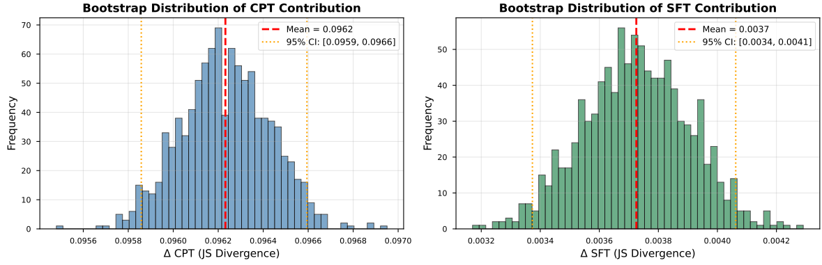
Figure 3: Bootstrap distribution of CPT and SFT contributions to JS divergence (1,000 iterations). Both distributions are narrow and exclude zero, confirming statistical robustness. Left: \Delta CPT = 0.096 [0.096, 0.097]. Right: \Delta SFT = 0.004 [0.003, 0.004].
