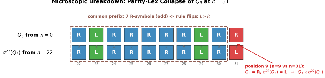
Figure 1: Parity-lex breakdown of Q_3 at n = 31 . The shaded common prefix contains seven R symbols (odd), flipping the order rule; at position 9 the candidate Q_3 emits R while \sigma^{22}(Q_3) emits L , so Q_3 \prec \sigma^{22}(Q_3) in the flipped order.
