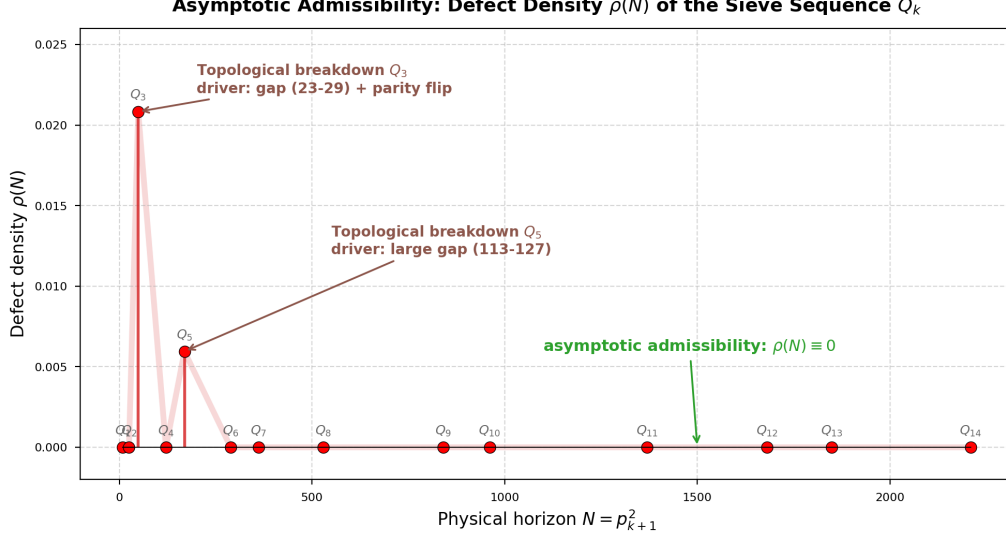
Figure 4: Topological defect density \rho(N) for Q_k , k = 1, \dots, 14 . Spikes at Q_3 ( n = 31 , parity flip) and Q_5 (the 113–127 gap) are crushed to zero for k \geq 6 by the topological shield.
