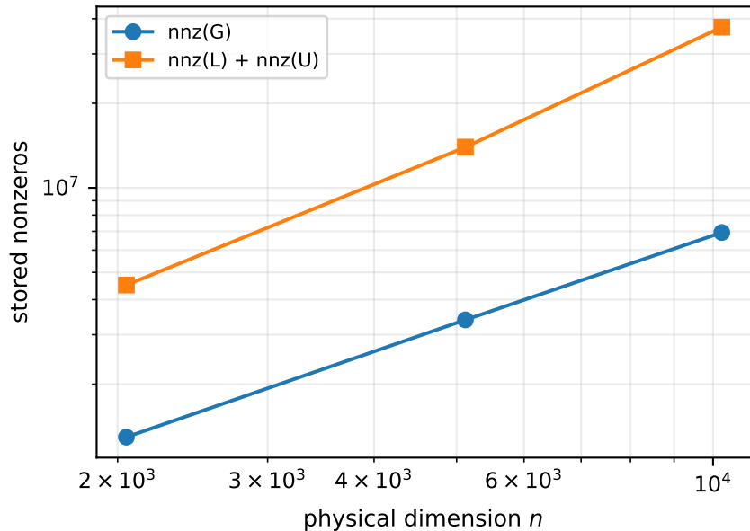
Sparse storage grows mildly on three pilot scales
