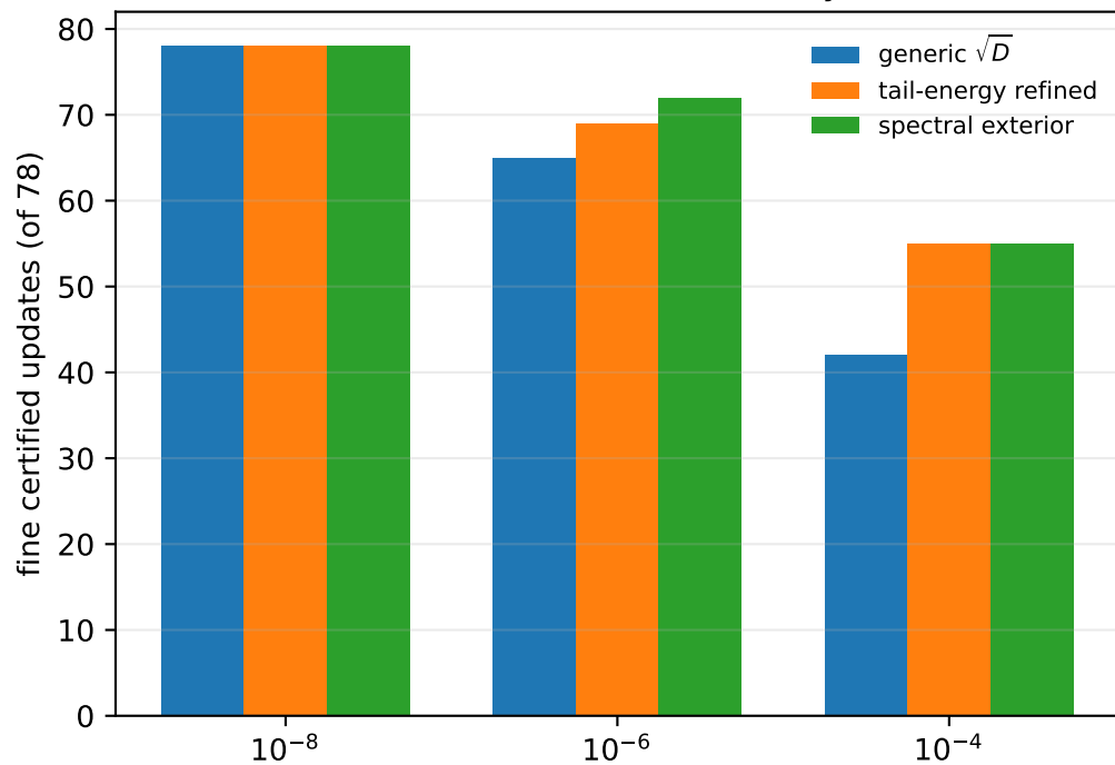
Trace certificate recovery
