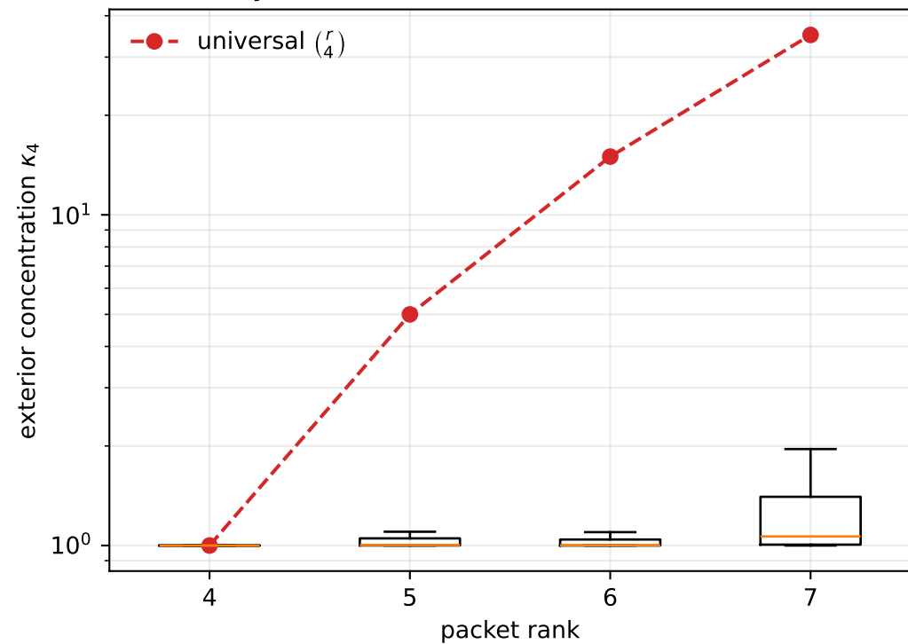
Physical concentration versus worst case
