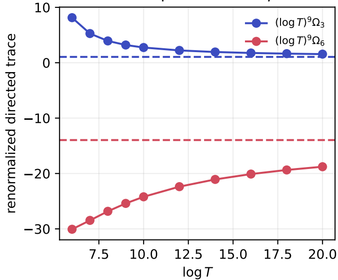
Macroscopic schedule, p = 2
