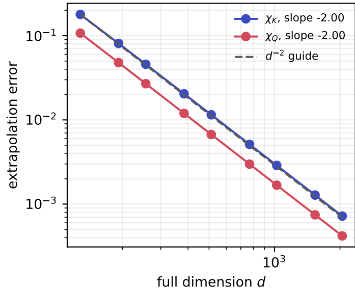
Curvature continuum limit
