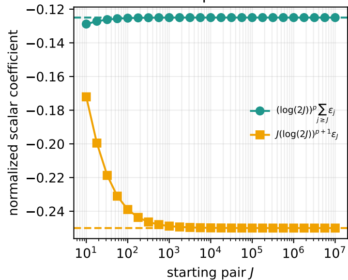
Summable pair-order tail
