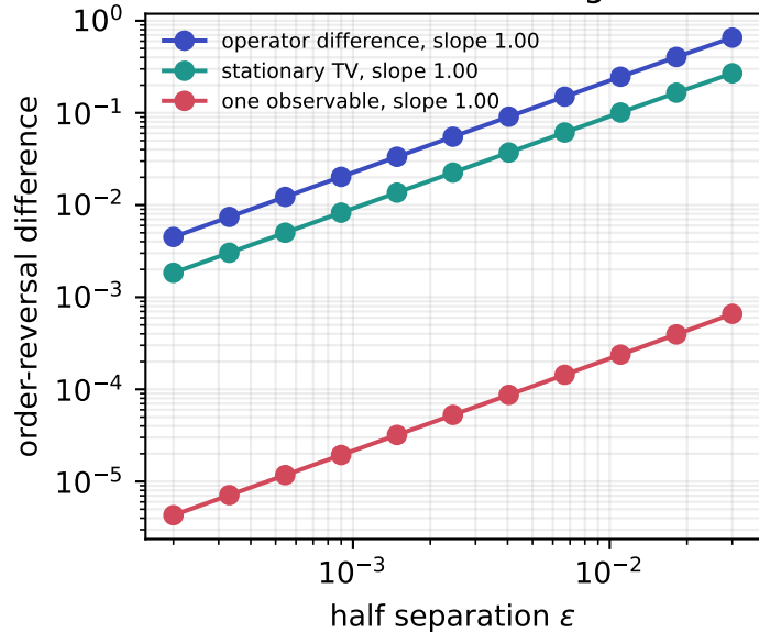
Order survives outside eigenvalues
