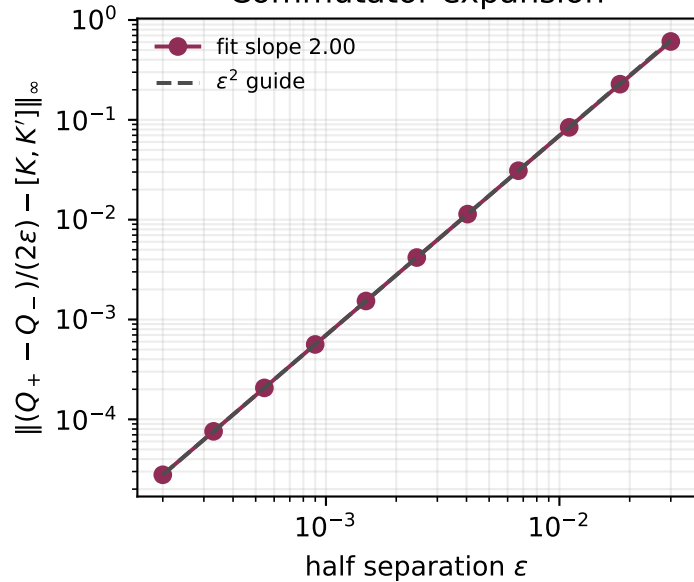
Commutator expansion
