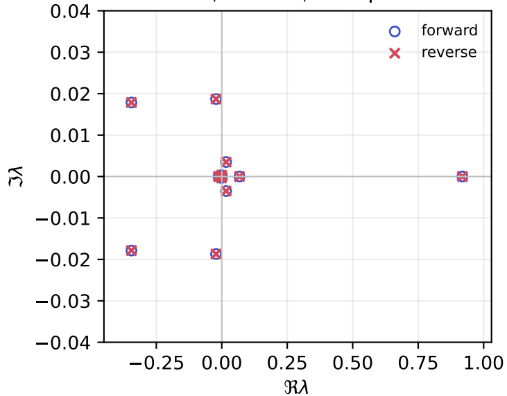
K_-K_+ and K_+K_- spectra
