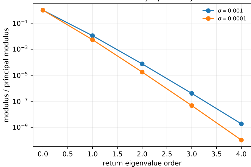
The branch return is asymptotically rank one
