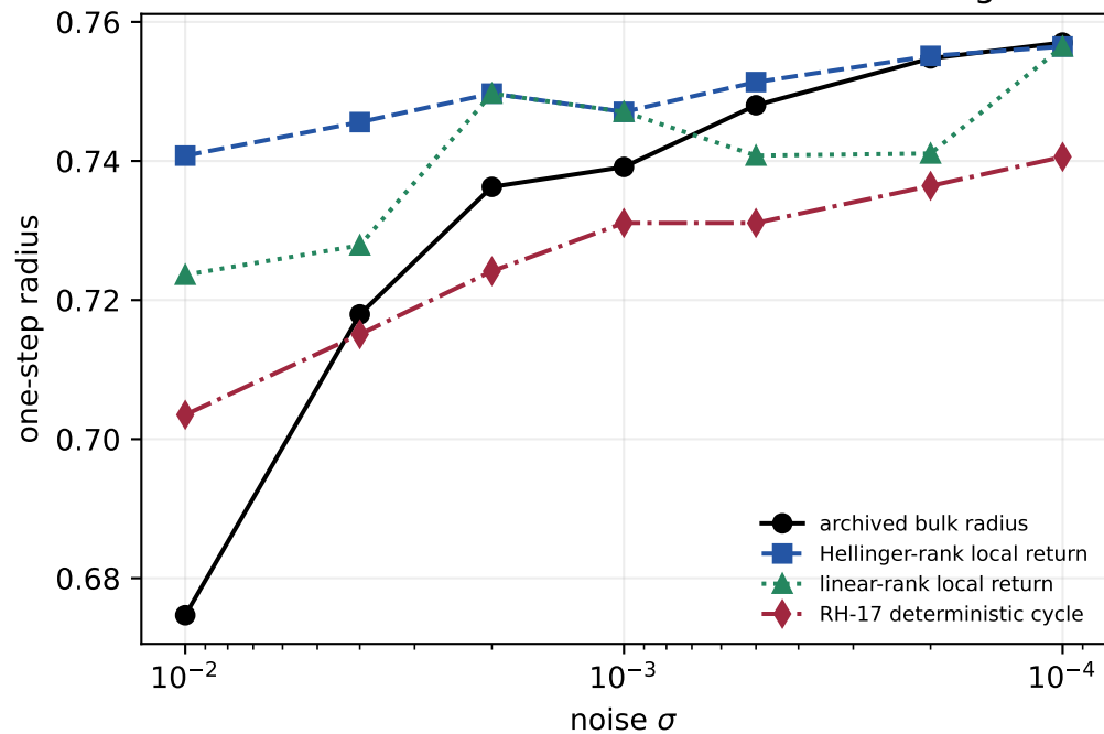
Branch-isolated return locates the bulk edge
