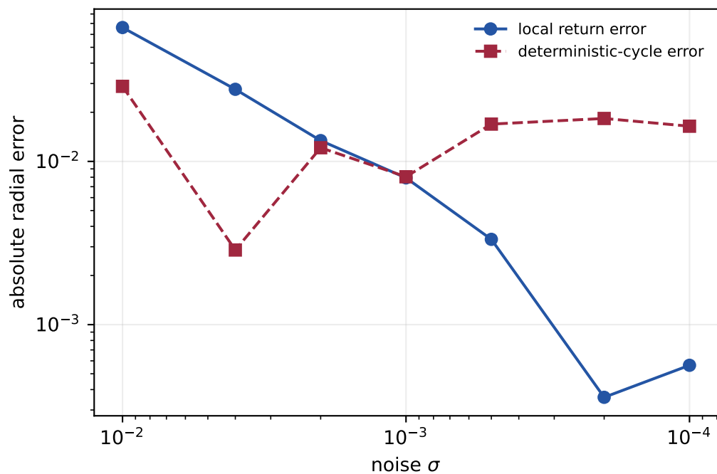
The nonlinear local correction wins in the tail
