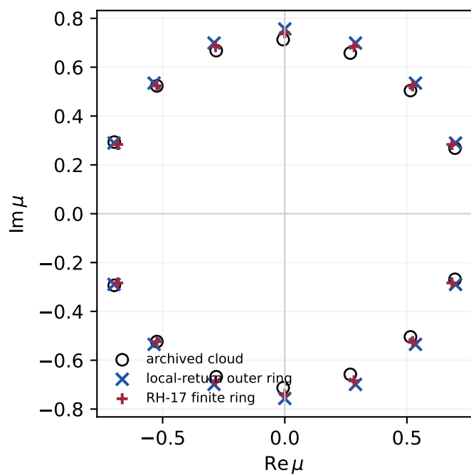
Two radial roles at \sigma = 0.0001
