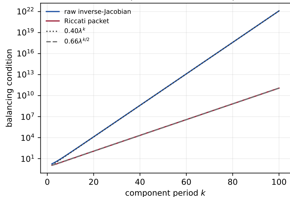
Gaussian adaptation halves the exponent
