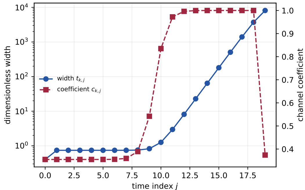
Periodic Riccati tube ( k = 20 )
