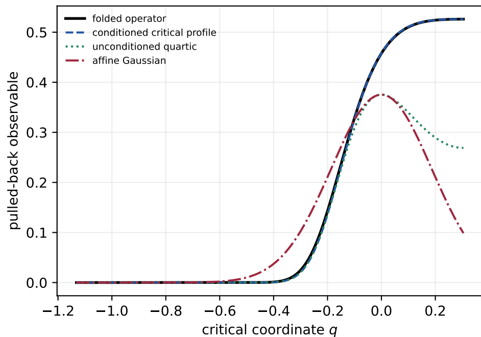
Critical closure at \sigma = 10^{-3}
