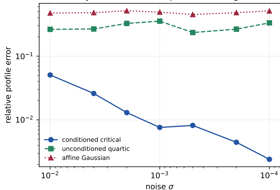
Only the conditioned profile converges
