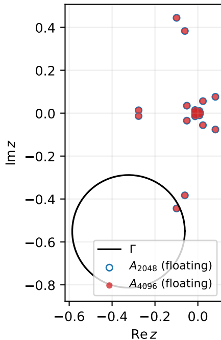
(c) Coarse physical resolvent atlas
