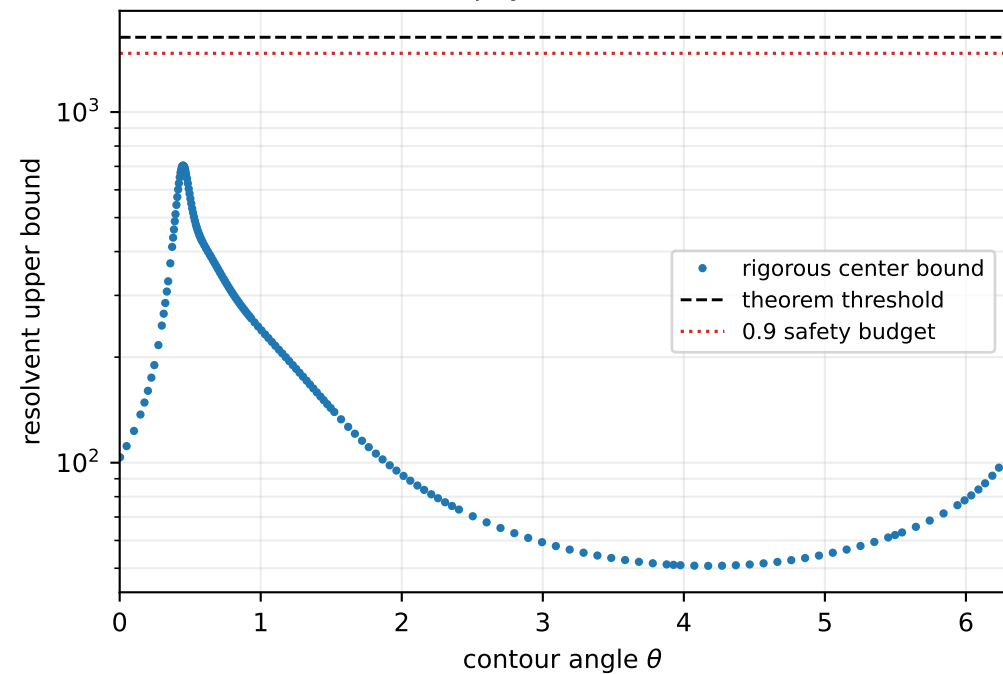
(c) Coarse physical resolvent atlas
