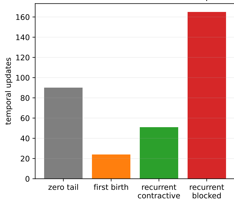
Relative-metric classification of 330 updates
