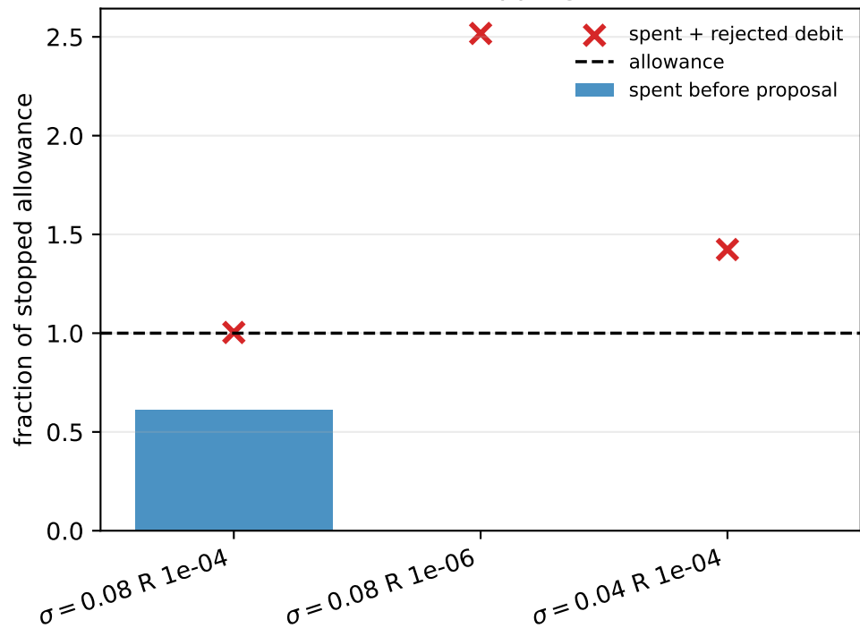
Three exact stopping events
