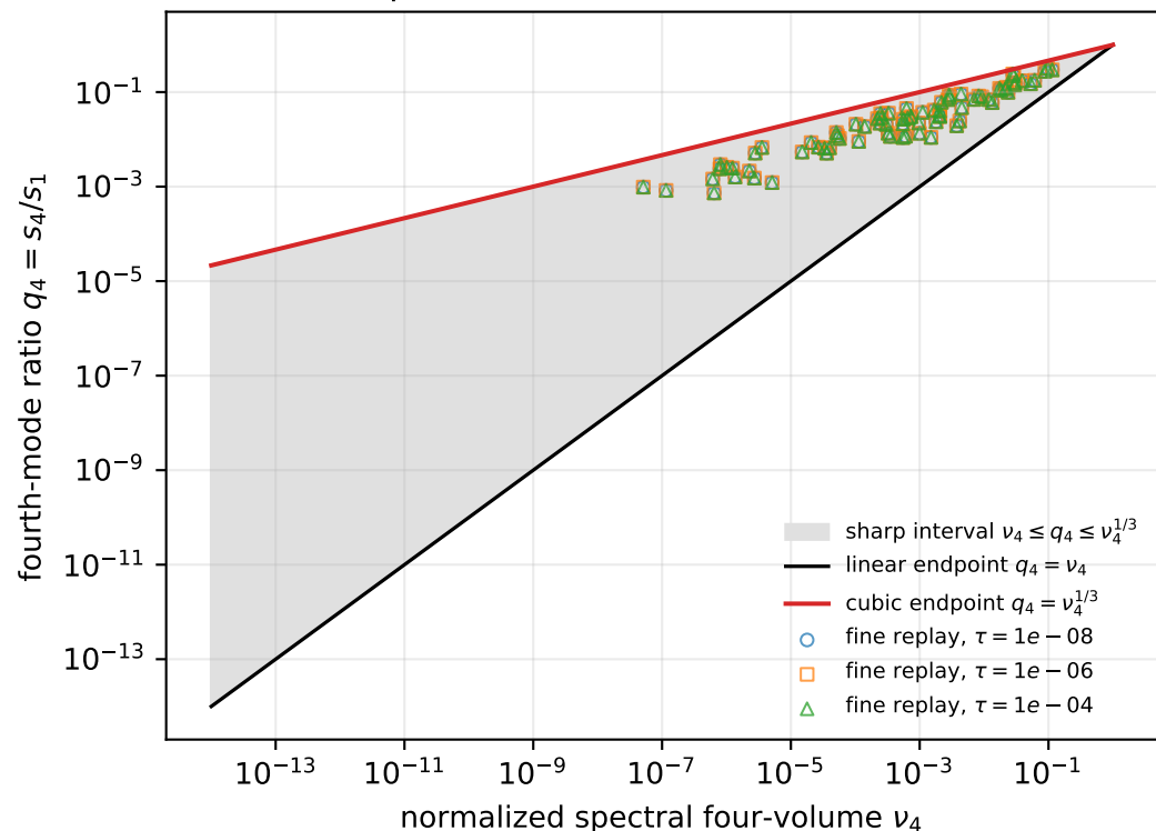
Sharp scalar-volume information barrier
