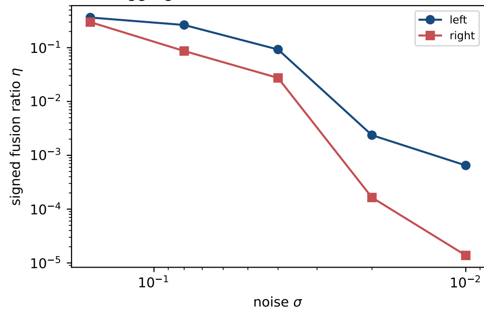
(c) Aggregate cancellation across radial blocks
