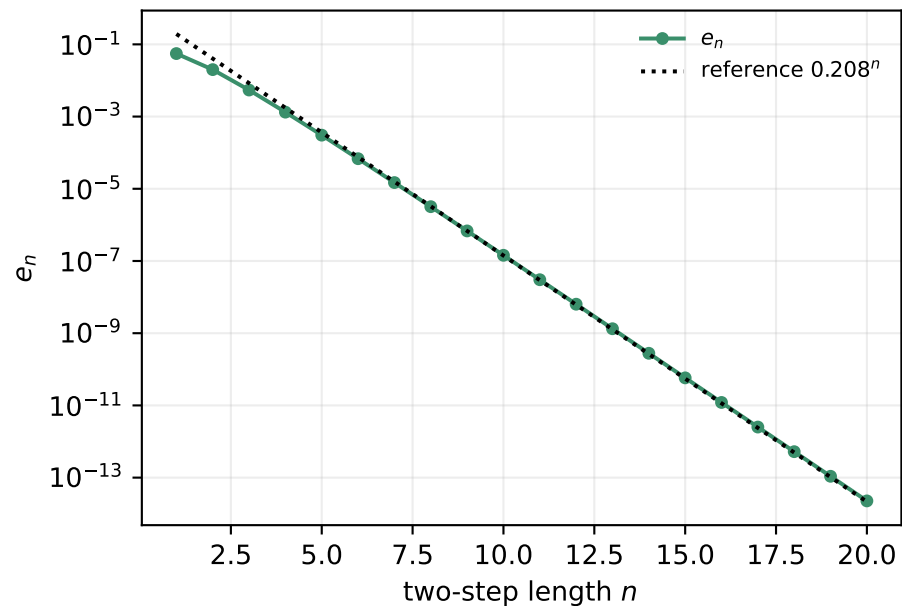
Deflated remainder
