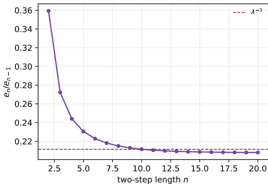
Remainder ratio
