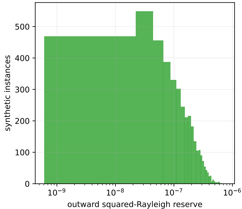
4,096 outward support bounds
