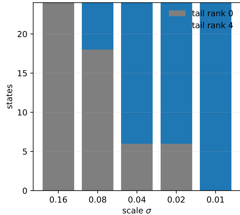
RH-130 semidefinite tail support
