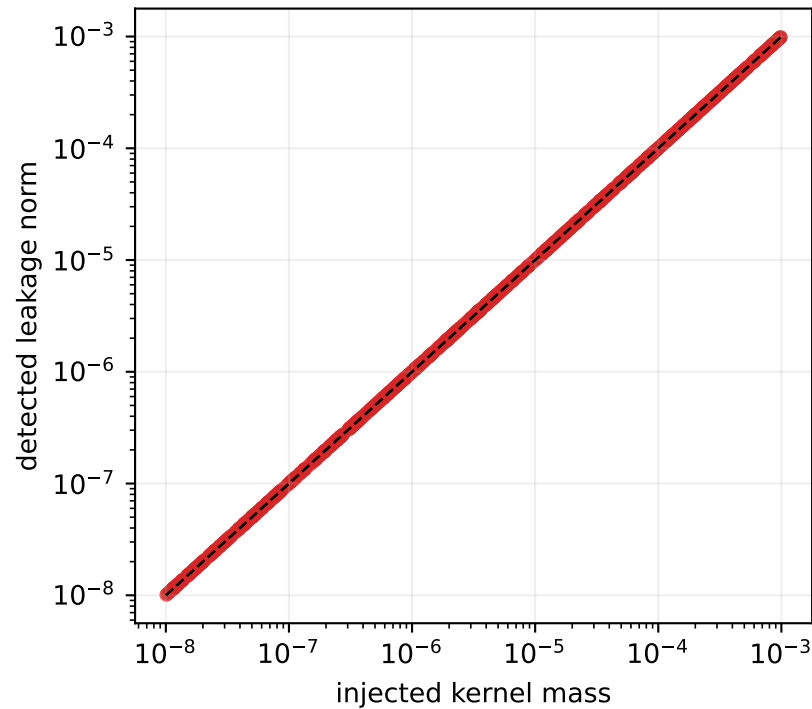
Any kernel leakage makes the full quotient infinite
