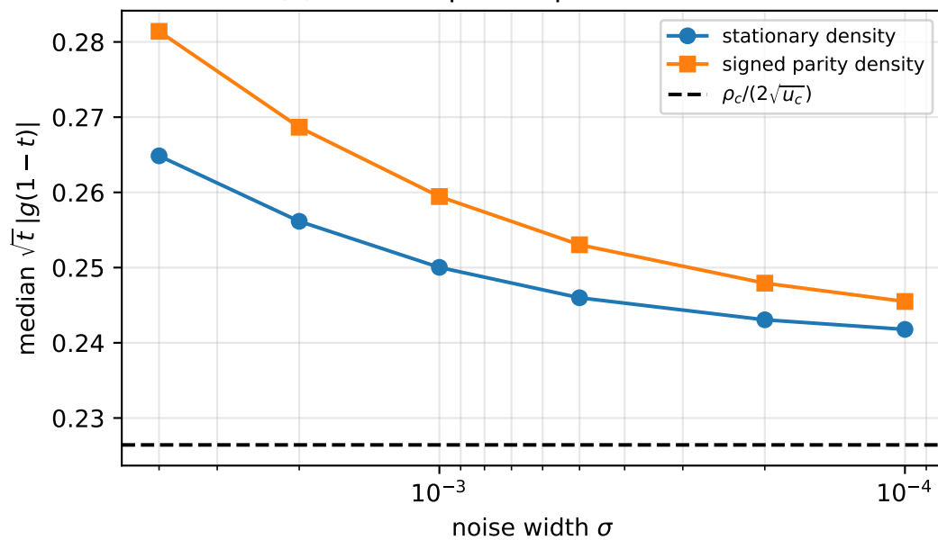
(c) Mesoscopic endpoint coefficient
