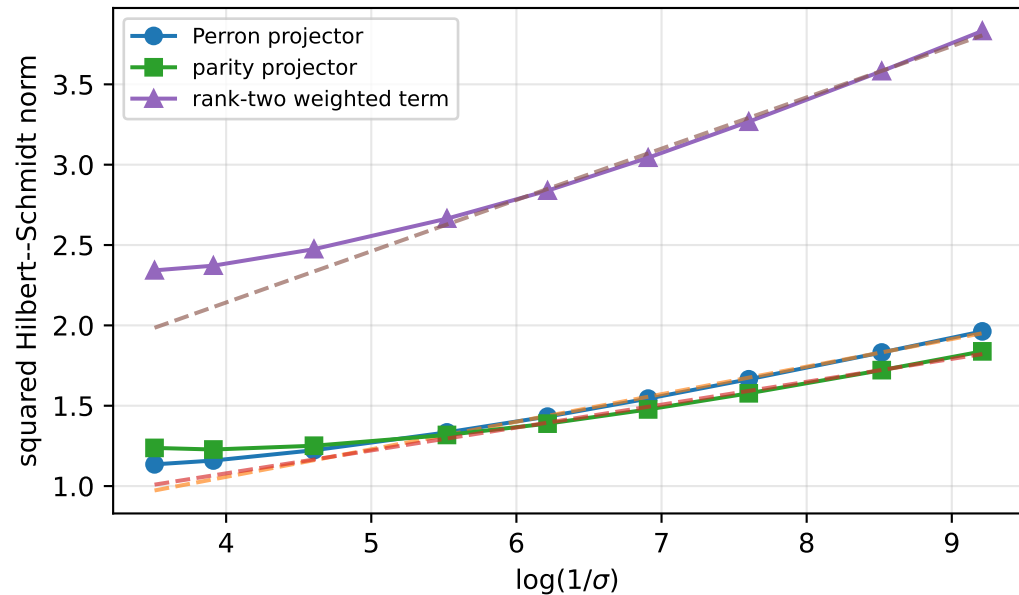
(a) Logarithmic peripheral growth
