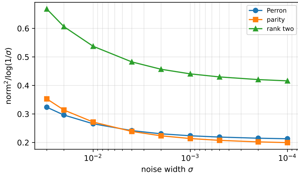
(b) Regular-variation index zero
