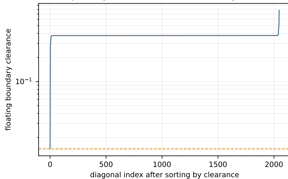
Dyadic signs are exact; distances are diagnostics
