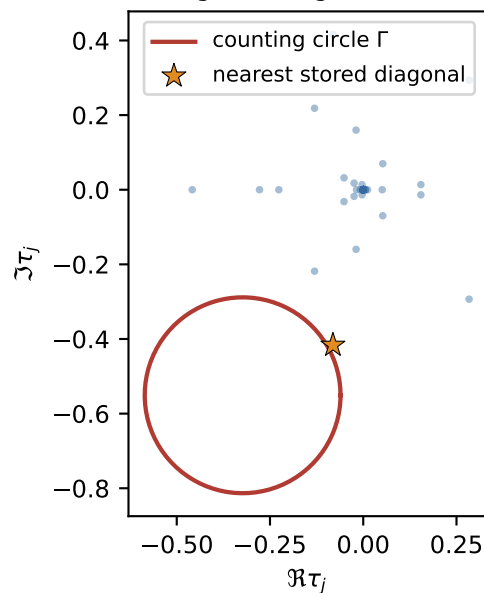
Exact stored triangular diagonal: 2048/2048 outside
