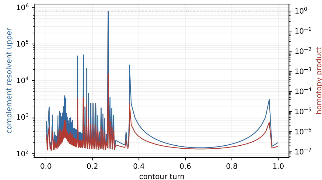
All 949 inherited rational leaves remain invertible
