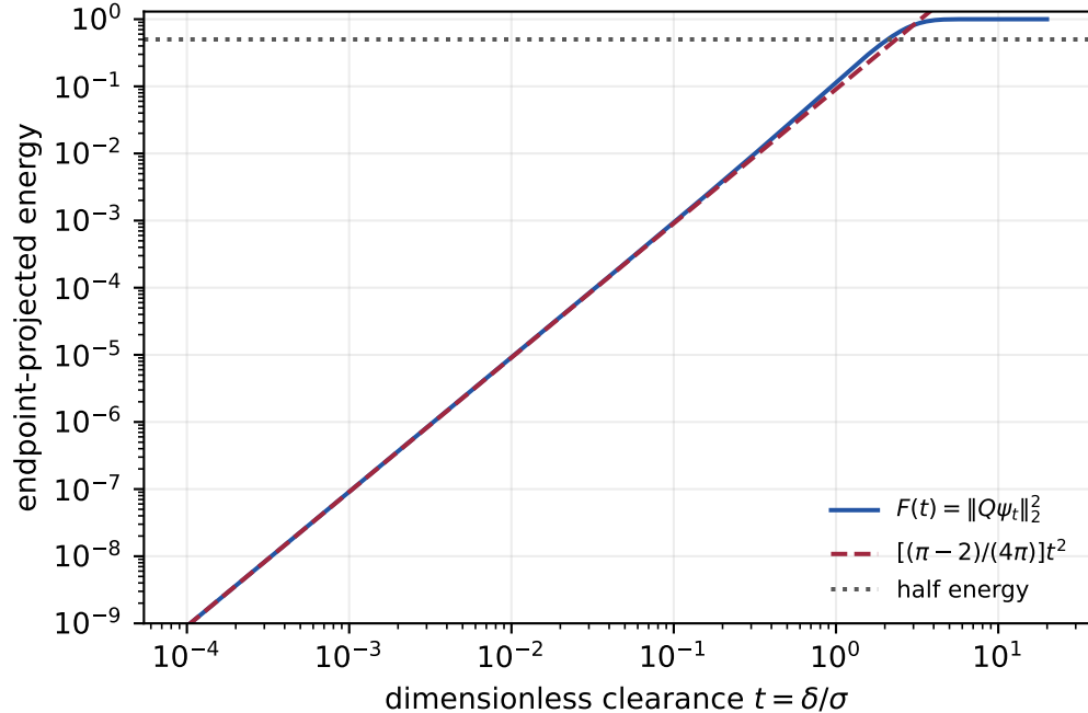
Exact conditioned-Gaussian transition
