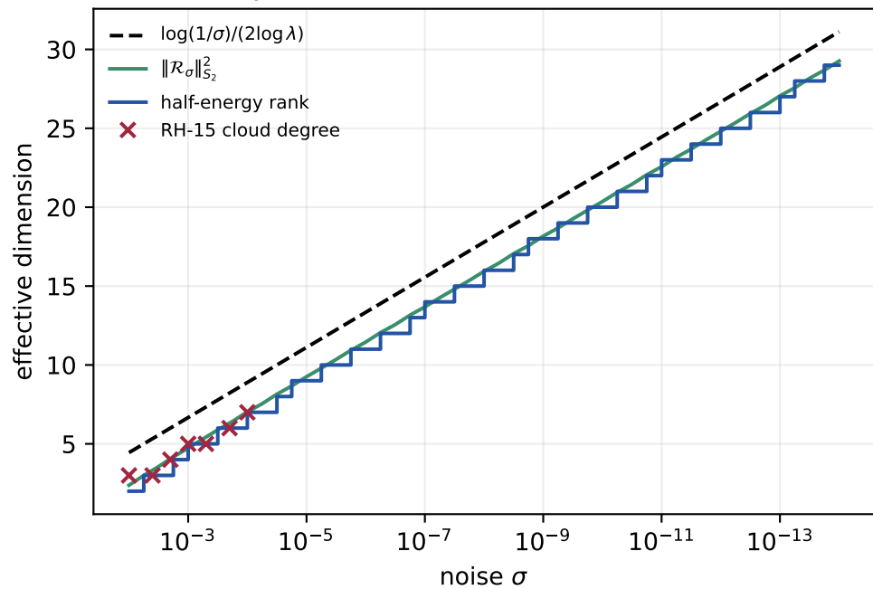
Analytic clock and archived cloud counts
