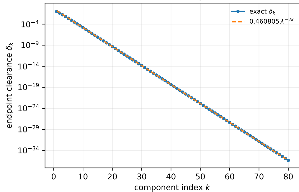
Geometric boundary ladder
