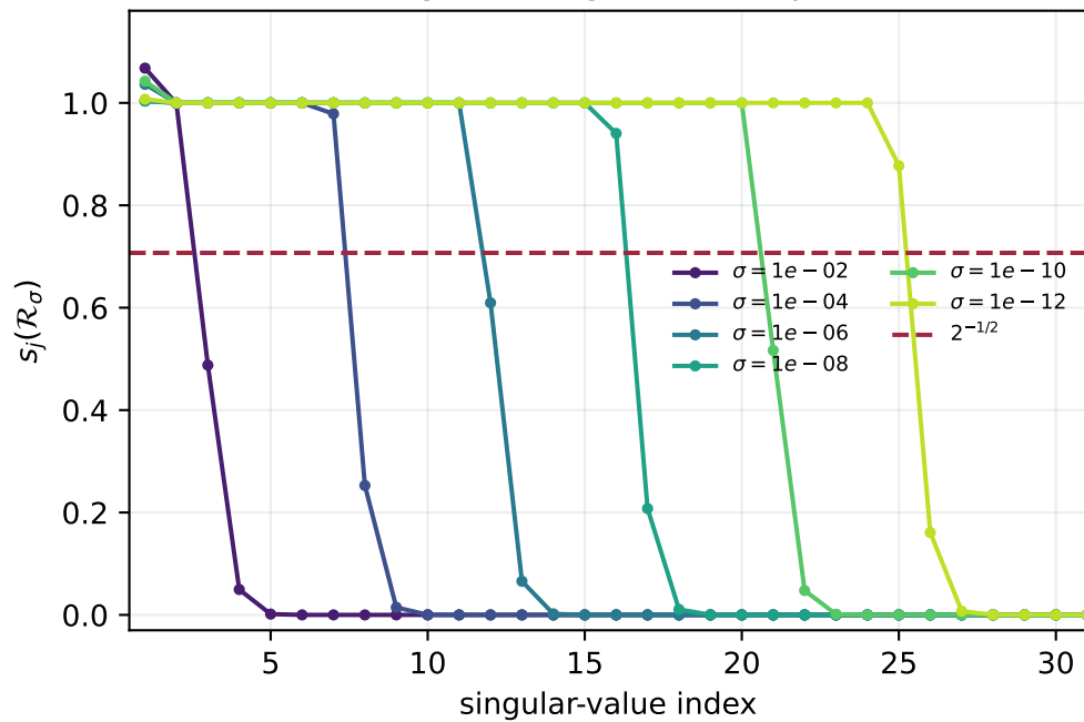
Growing unit singular-value plateau
