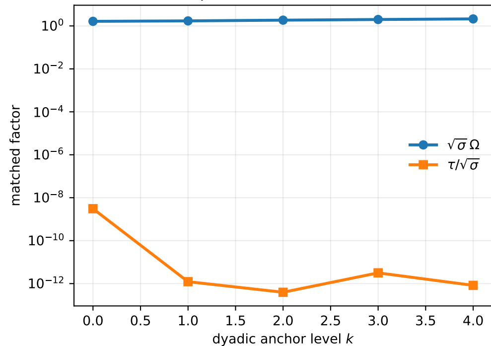
Square-root factorization
