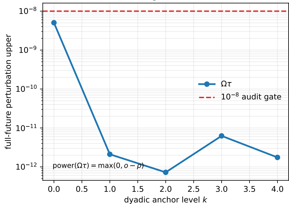
Observation growth is canceled
