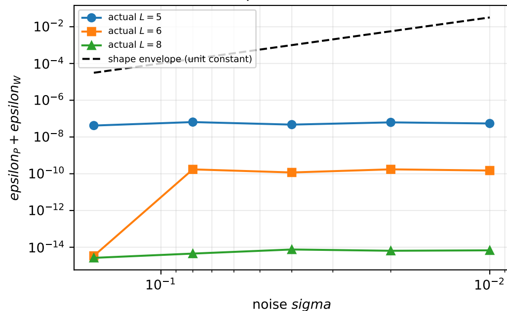
(b) Recomputed intrinsic factors
