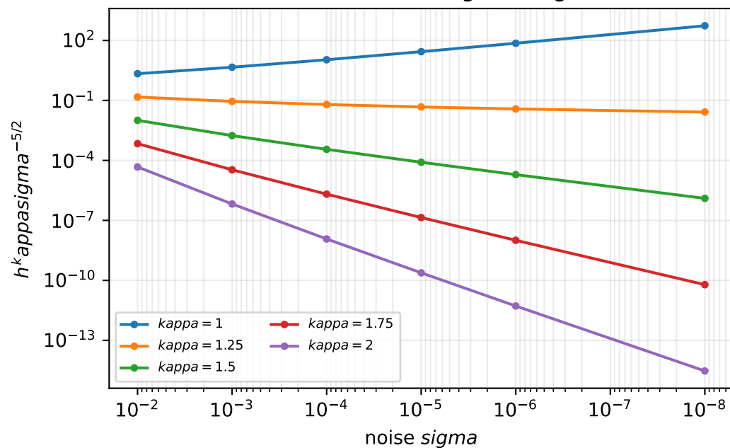
(c) Near-critical h = \sigma^2 / \log(1/\sigma)
