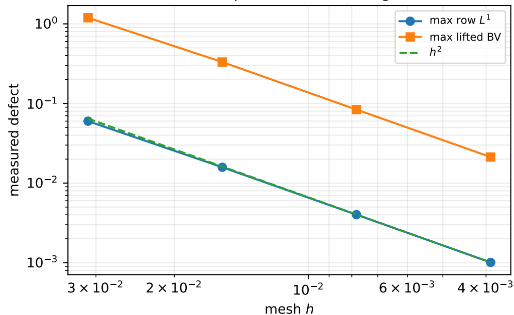
(a) Midpoint-to-Ulam bridge
