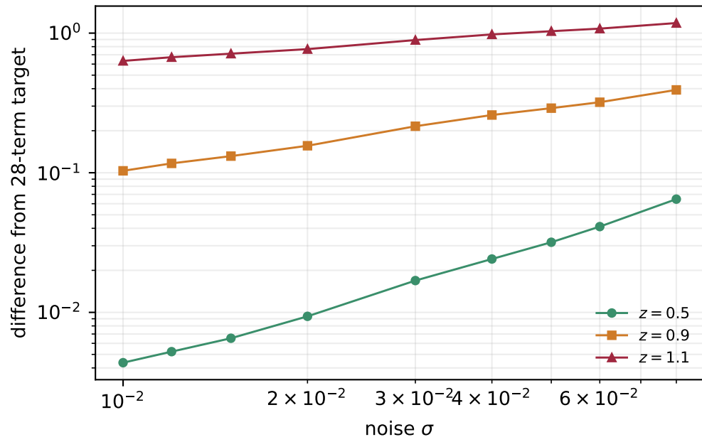
Coefficientwise approach, not uniformity
