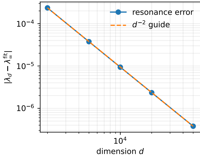
Isolated resonance
