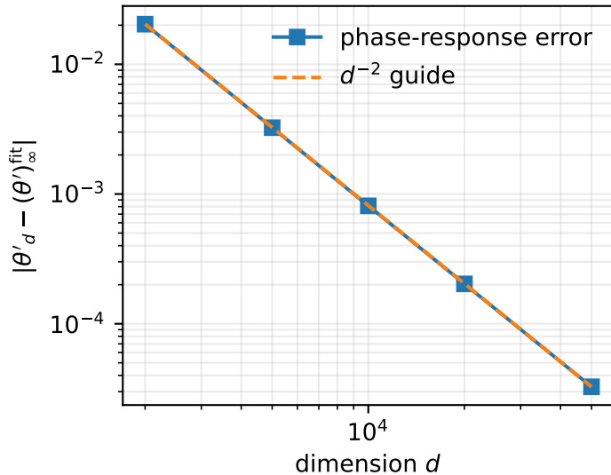
Derivative of eigenphase
