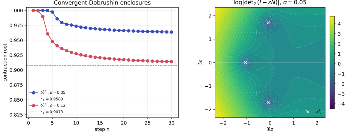
Figure 3: Left: multistep Dobrushin roots and finite-matrix non-Perron radii at u = u_c , d = 512 . The roots decrease toward the dashed spectral radii. Right: \log|\det_2(I - zN)| at \sigma = 0.05 , with crosses at reciprocals of resonances having modulus above 0.1.
