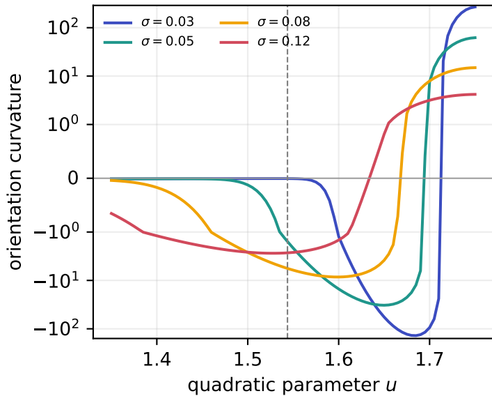
One-step curvature \chi_K
