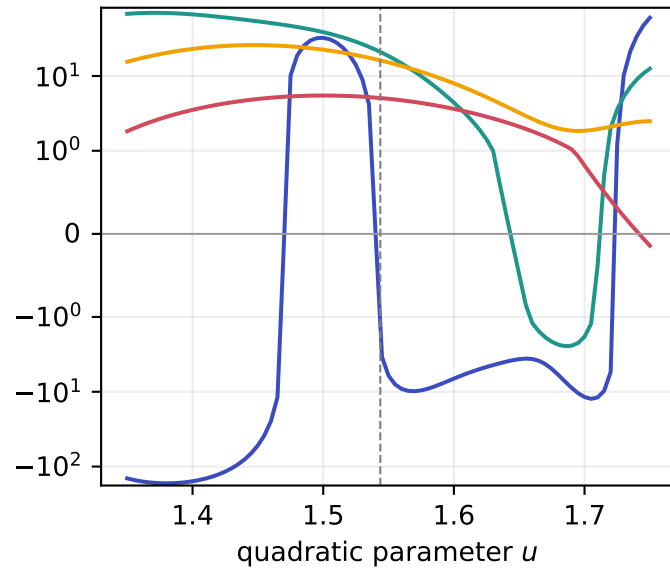
Parity-block curvature \chi_Q
