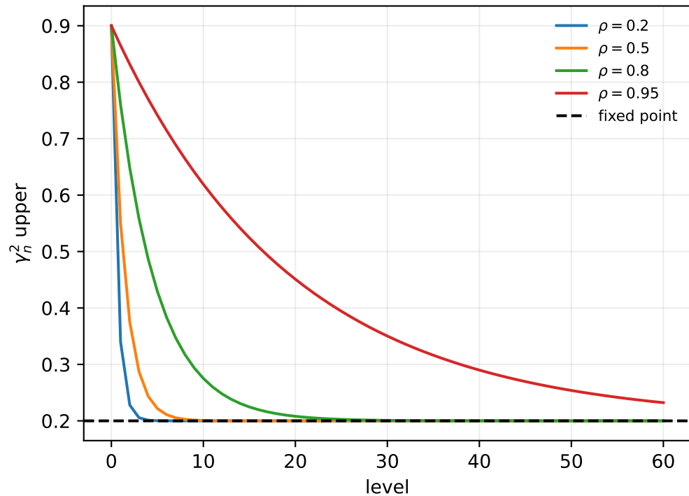
Contractive affine envelopes
