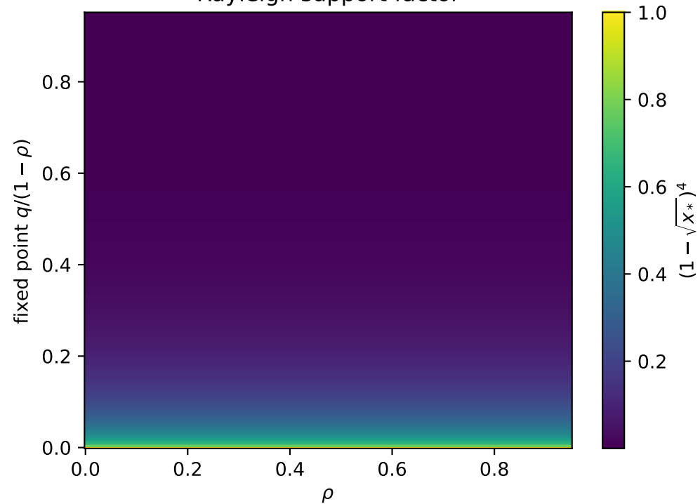
Rayleigh support factor
