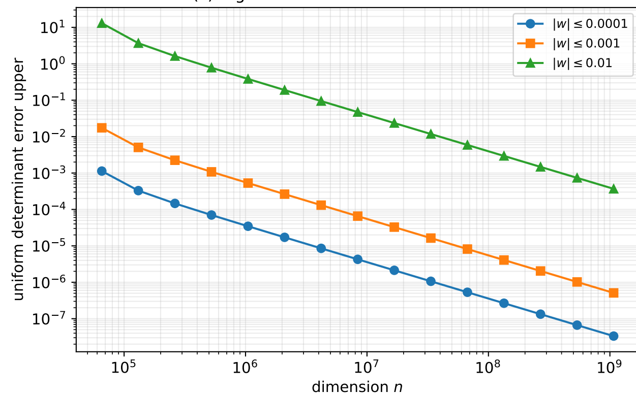
(c) Rigorous Fredholm determinant disks
