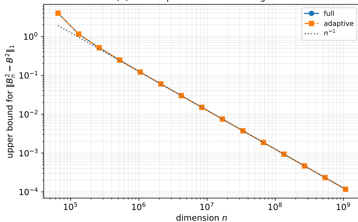
(b) Two-step trace-norm convergence
