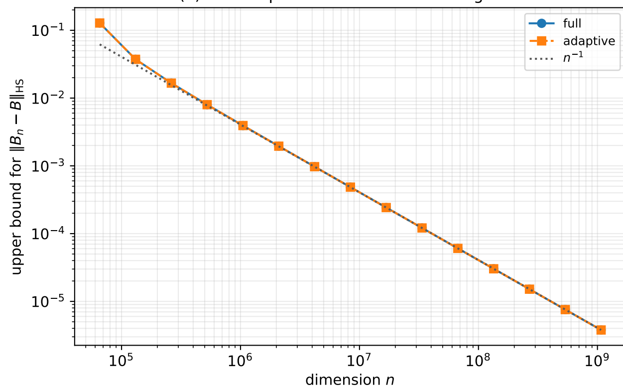
(a) One-step Hilbert--Schmidt convergence
