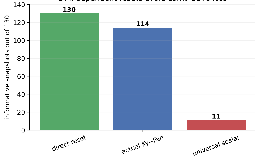
D. Independent resets avoid cumulative loss
