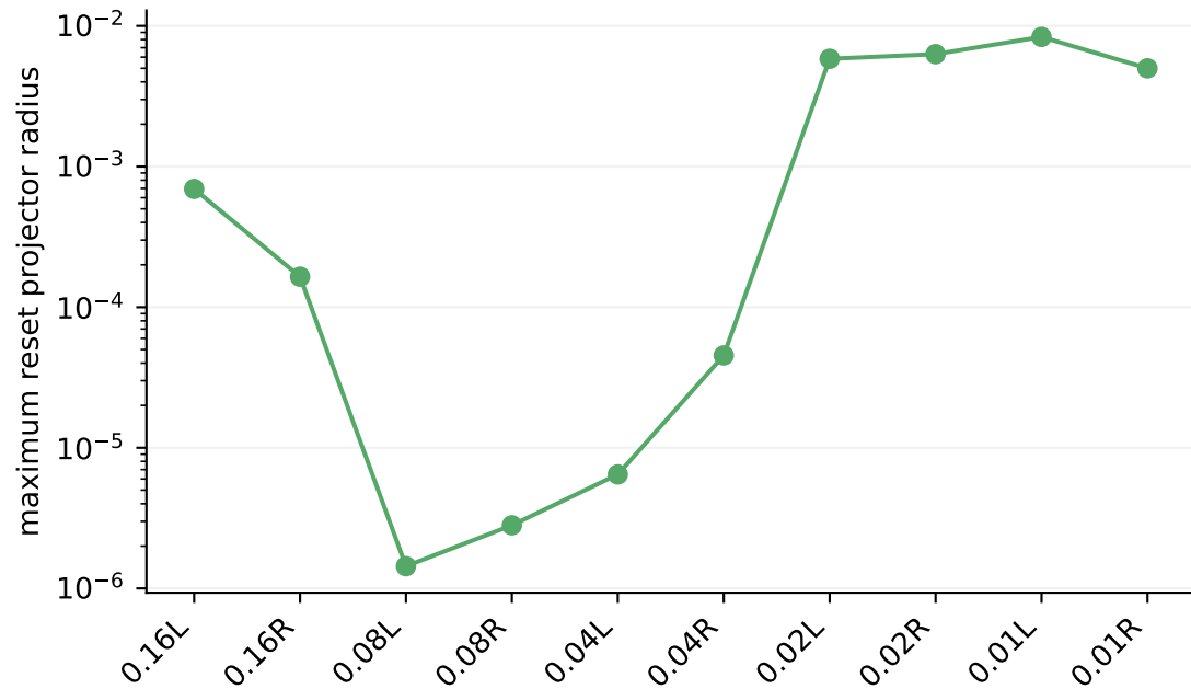
D. Independent resets avoid cumulative loss
