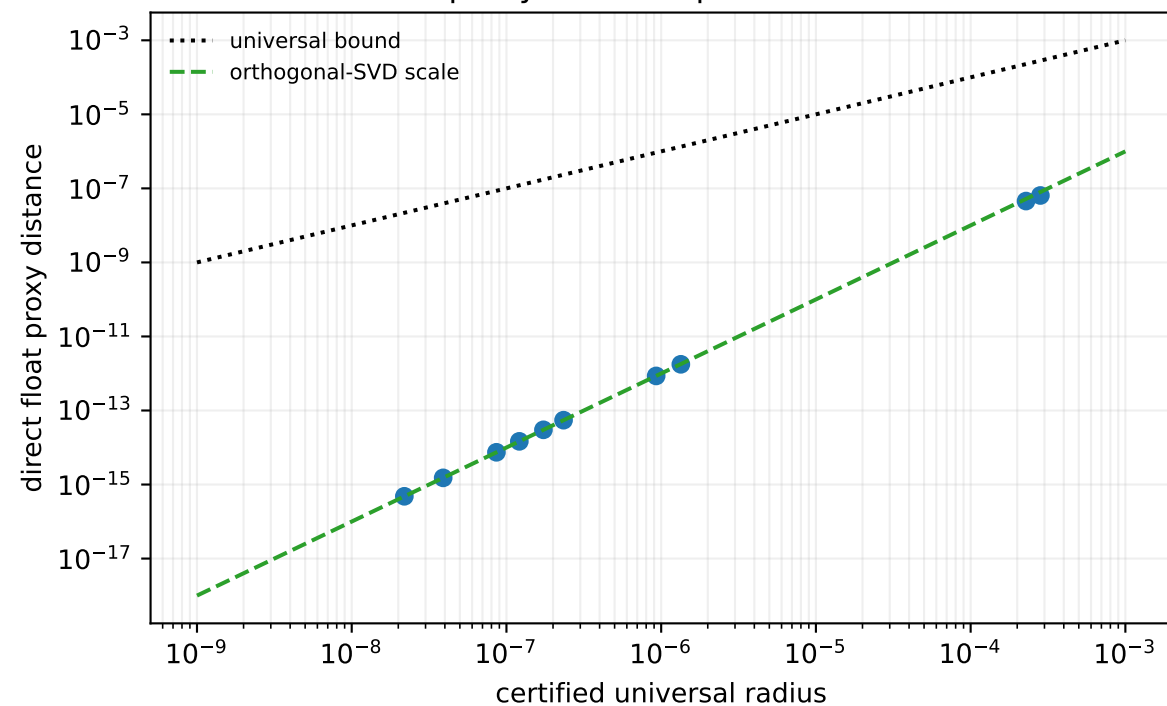
Rank-four proxy exhibits quadratic cancellation
