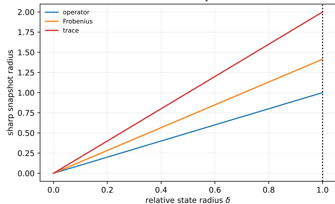
All constants are attained by one-row witnesses
