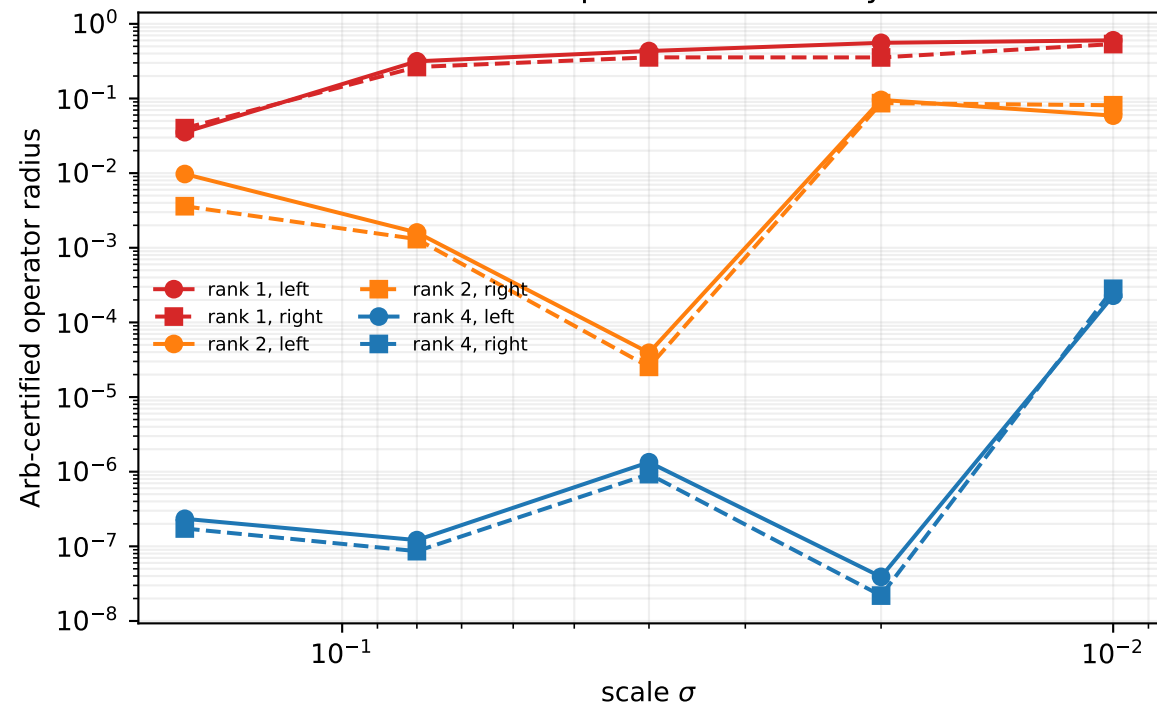
Normalized snapshot enclosure by rank
