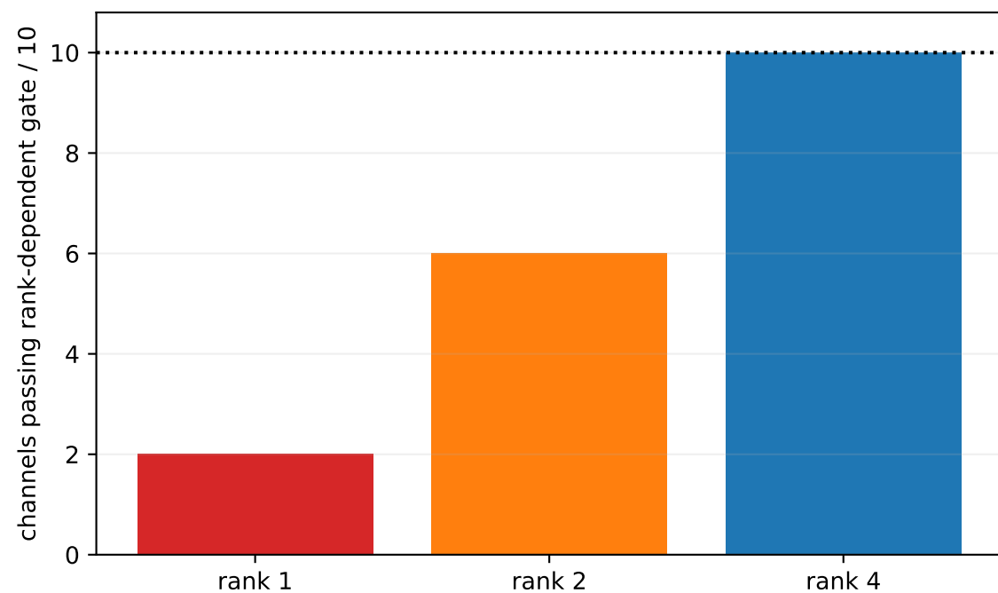
All rank-four balls are below 10^{-3}
