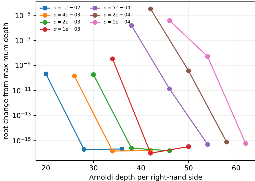
Projected root stabilization
