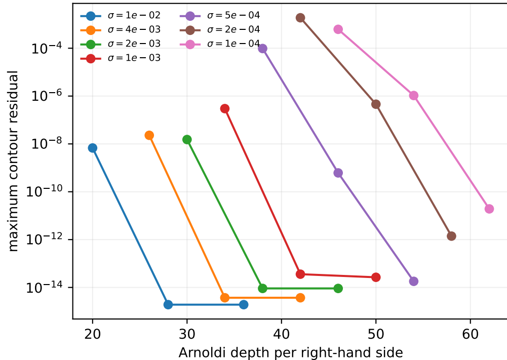
Holomorphic shifted-solve convergence
