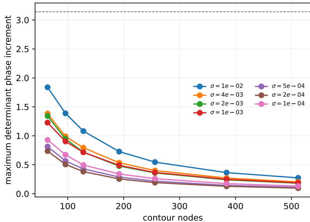
Phase sampling remains well below \pi
