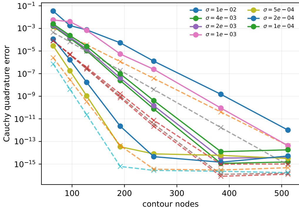
Count (circles) and centroid (crosses) converge
