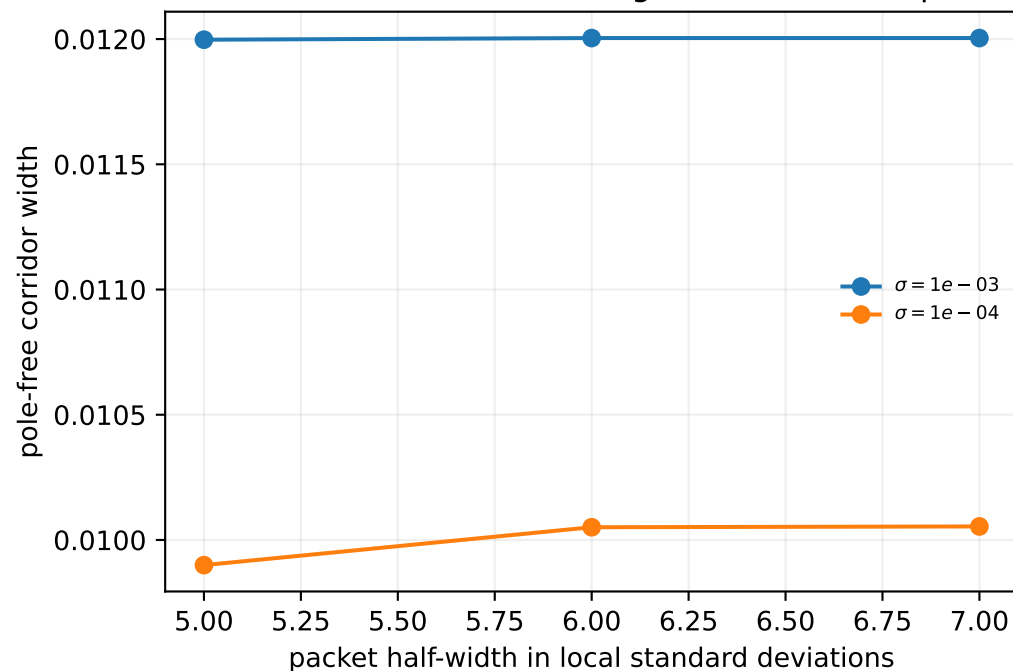
The isolation corridor changes but remains open
