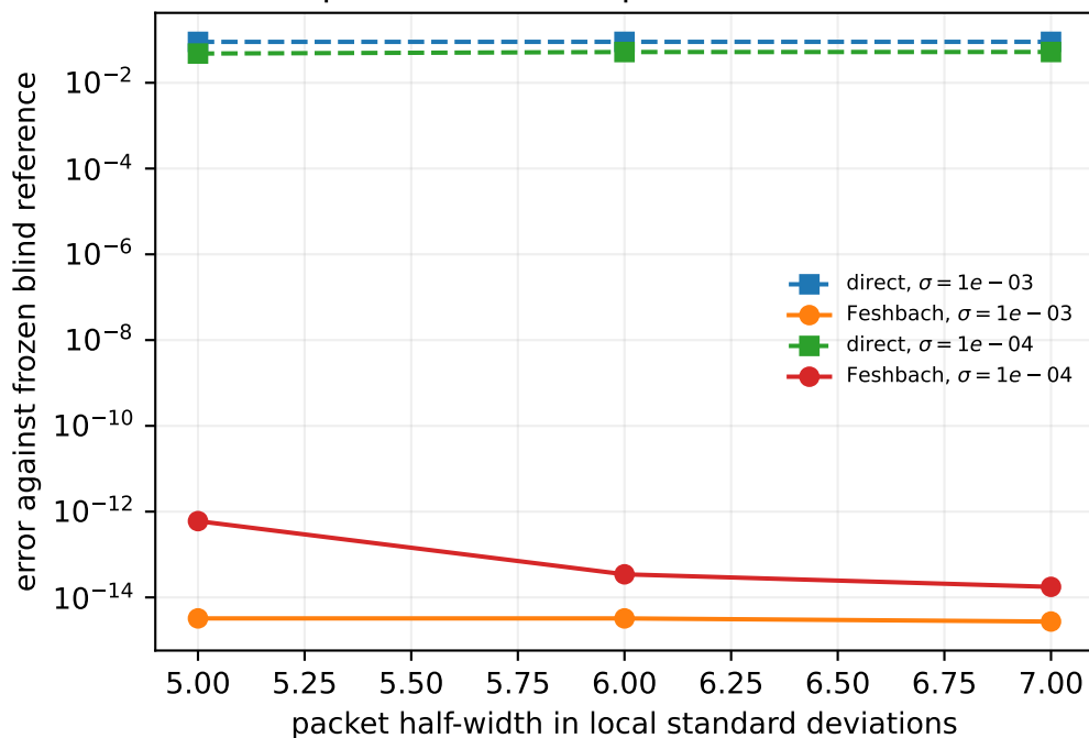
The predicted root is packet-window stable
