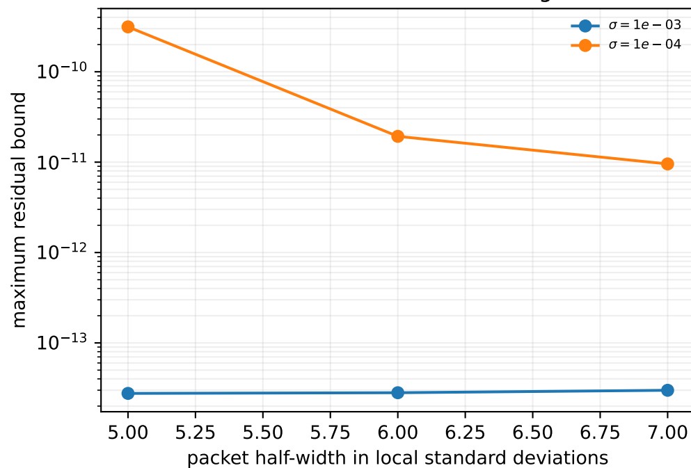
Shifted solves remain converged
