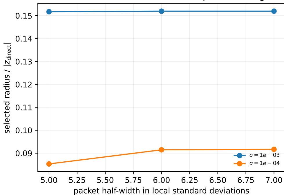
Contour renormalization absorbs packet changes
