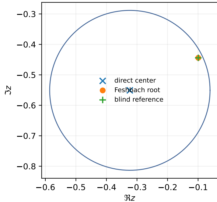
One-root contour, \sigma = 1e-02
