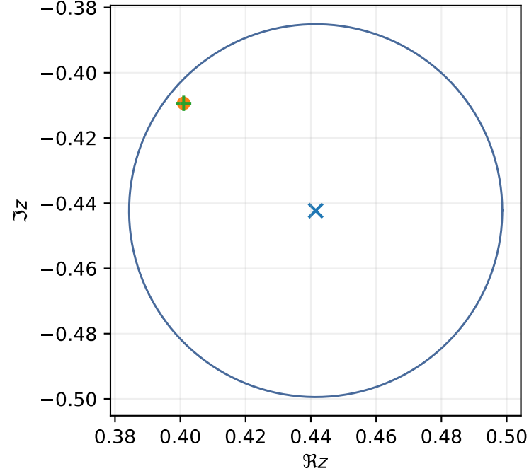
One-root contour, \sigma = 1e-04
