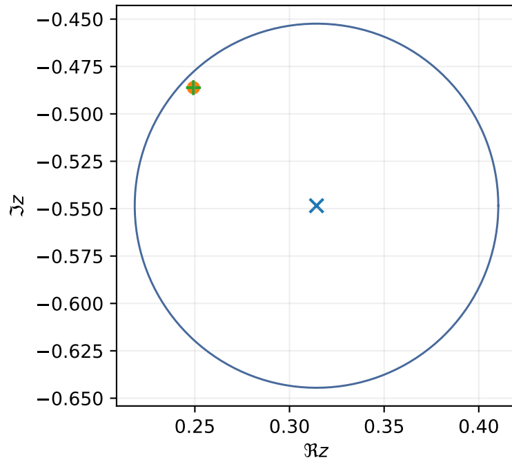
One-root contour, \sigma = 1e-03
