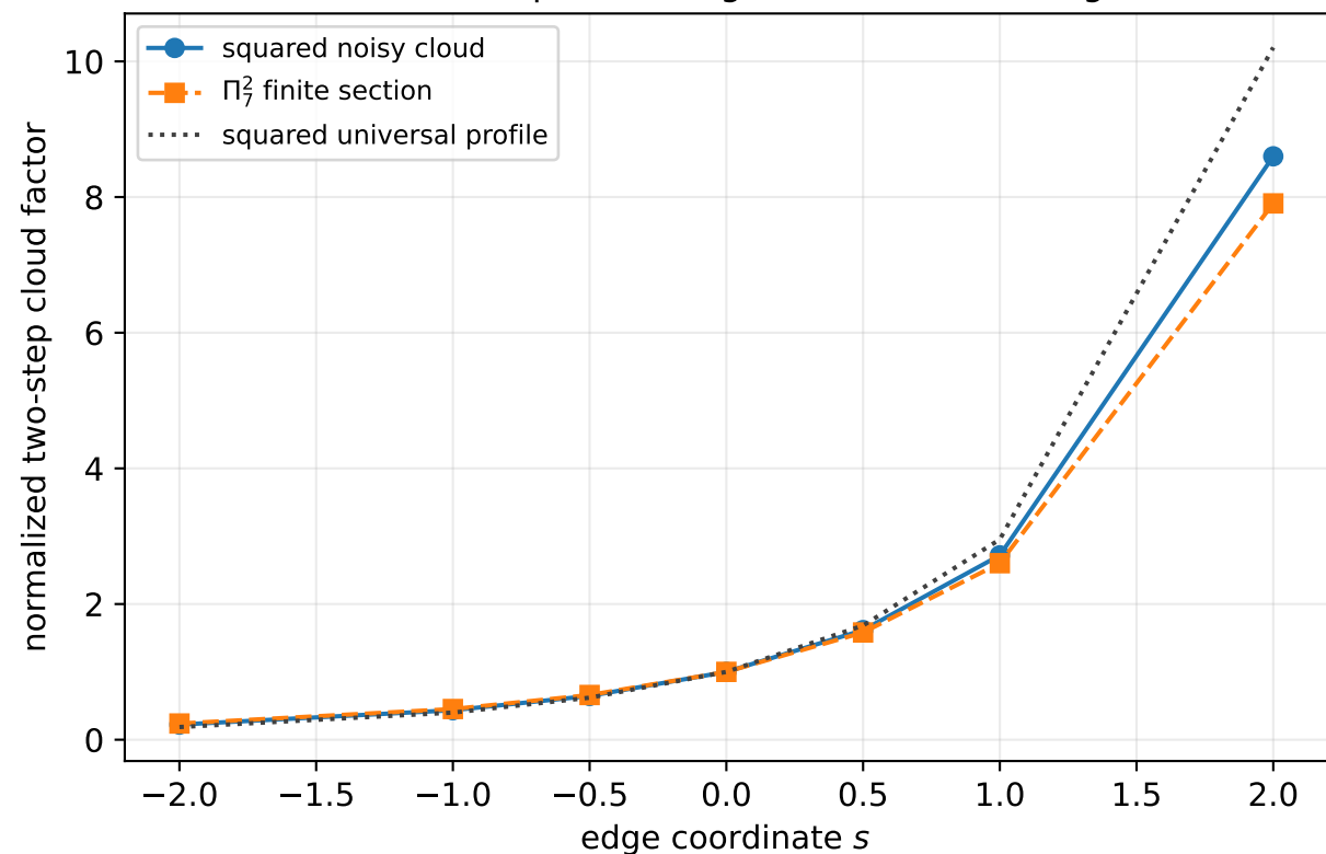
(d) Two-step scattering at \sigma = 10^{-4} (floating)
