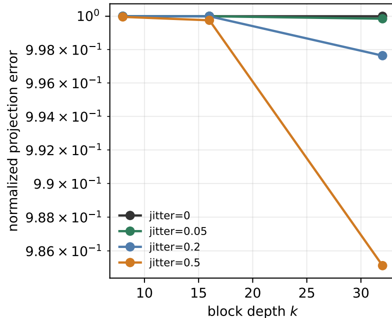
Perturbed rings remain hard
