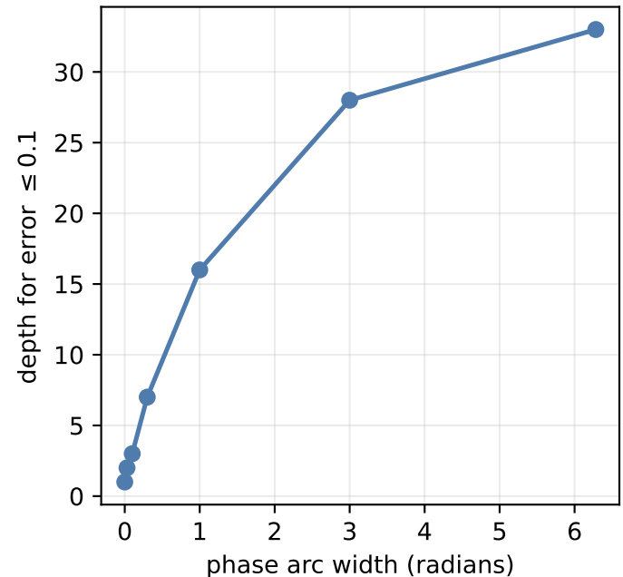
Phase compression opens the route
