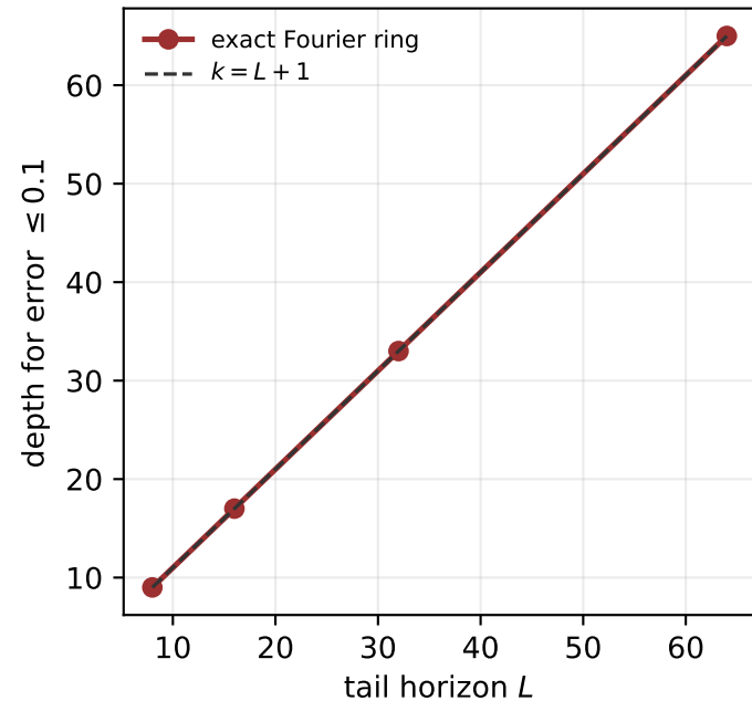
Exact depth obstruction
