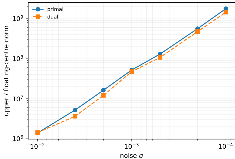
Residual inflation
