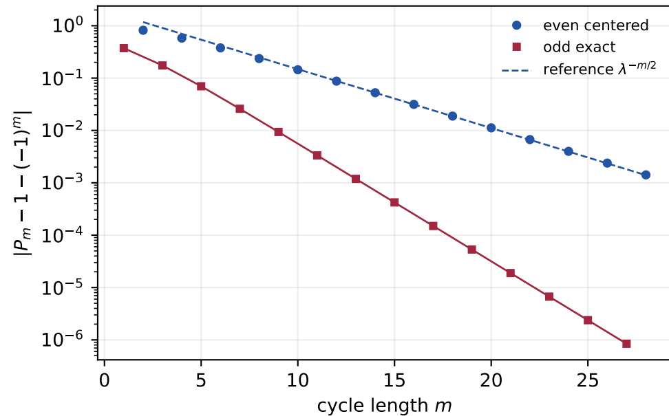
Parity-centered decay
