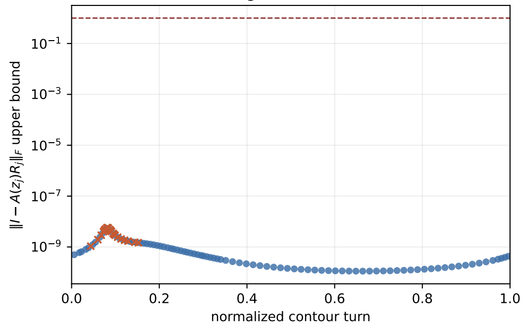
Exact-target residual recheck
