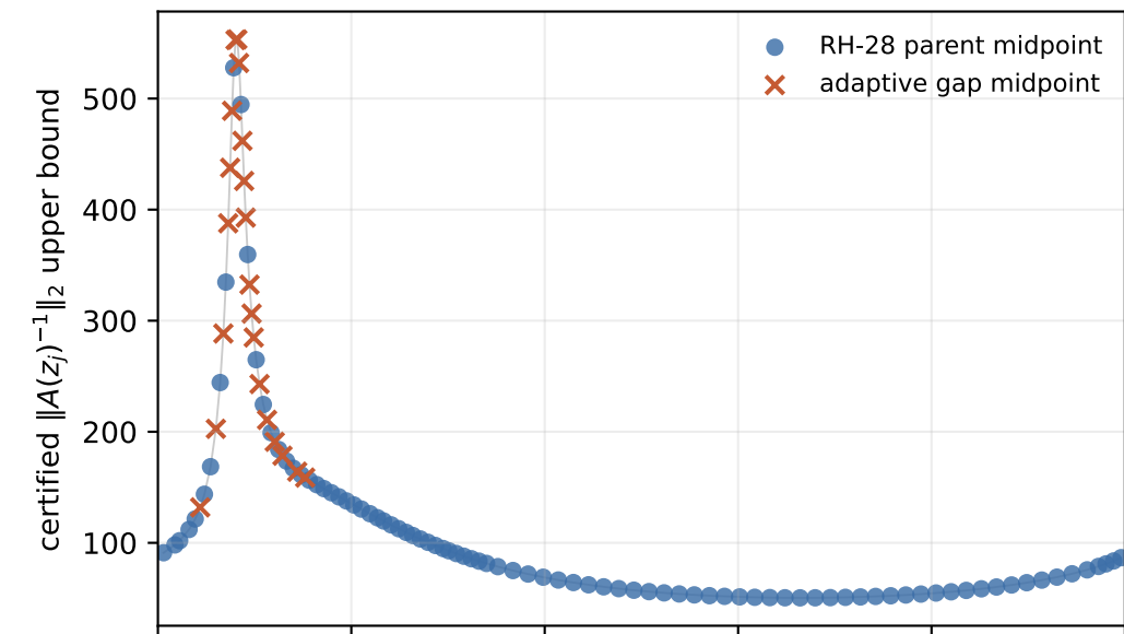
109 direct center certificates
