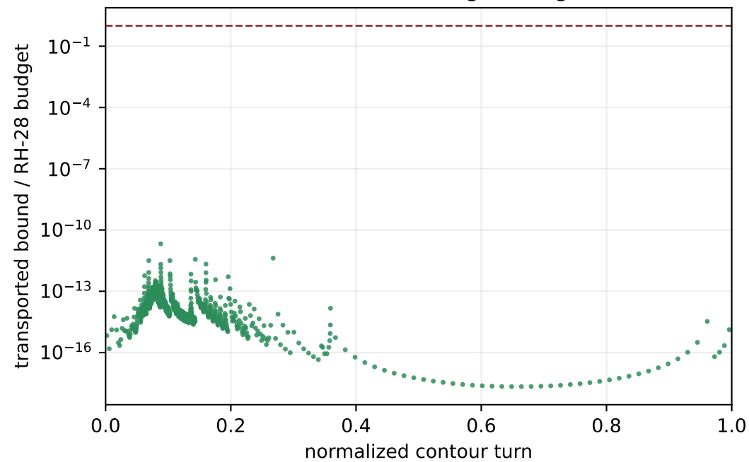
Arcwise Rouché-budget margins
