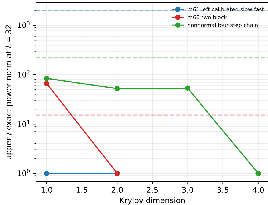
Residual certificate versus ordinary norm
