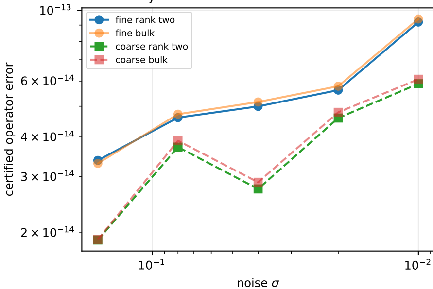
Projector and deflated-bulk enclosure
