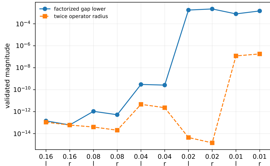
All ten packet gaps remain open
