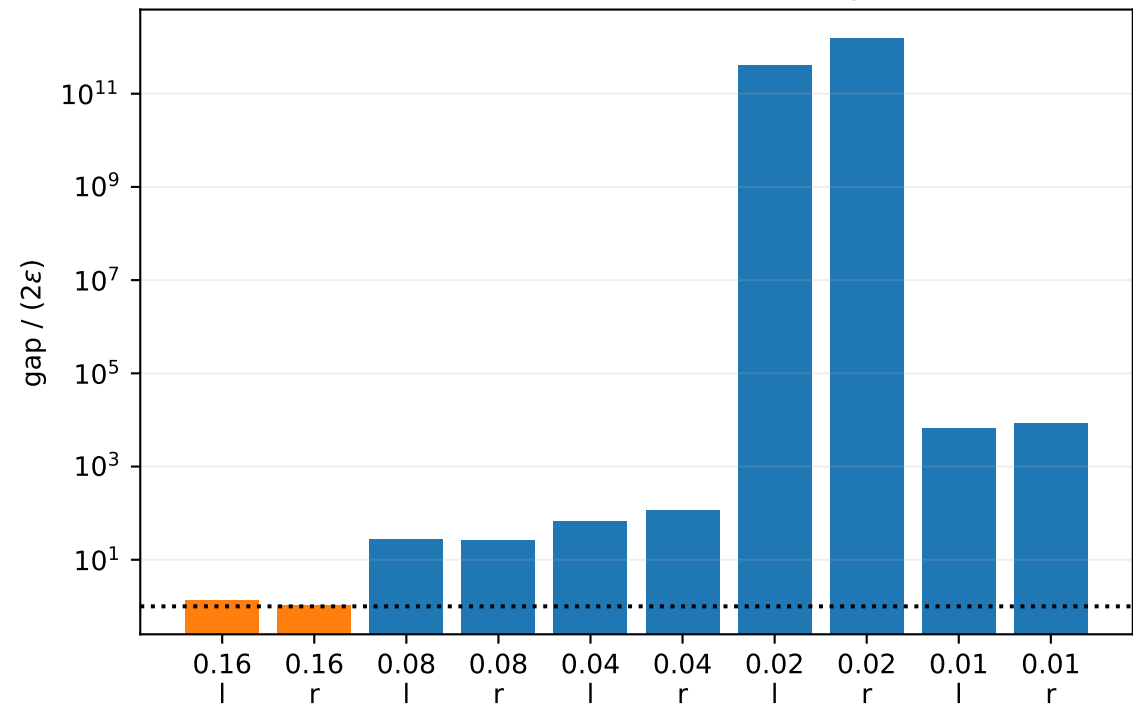
Two coarse channels need interval-eigen rescue
