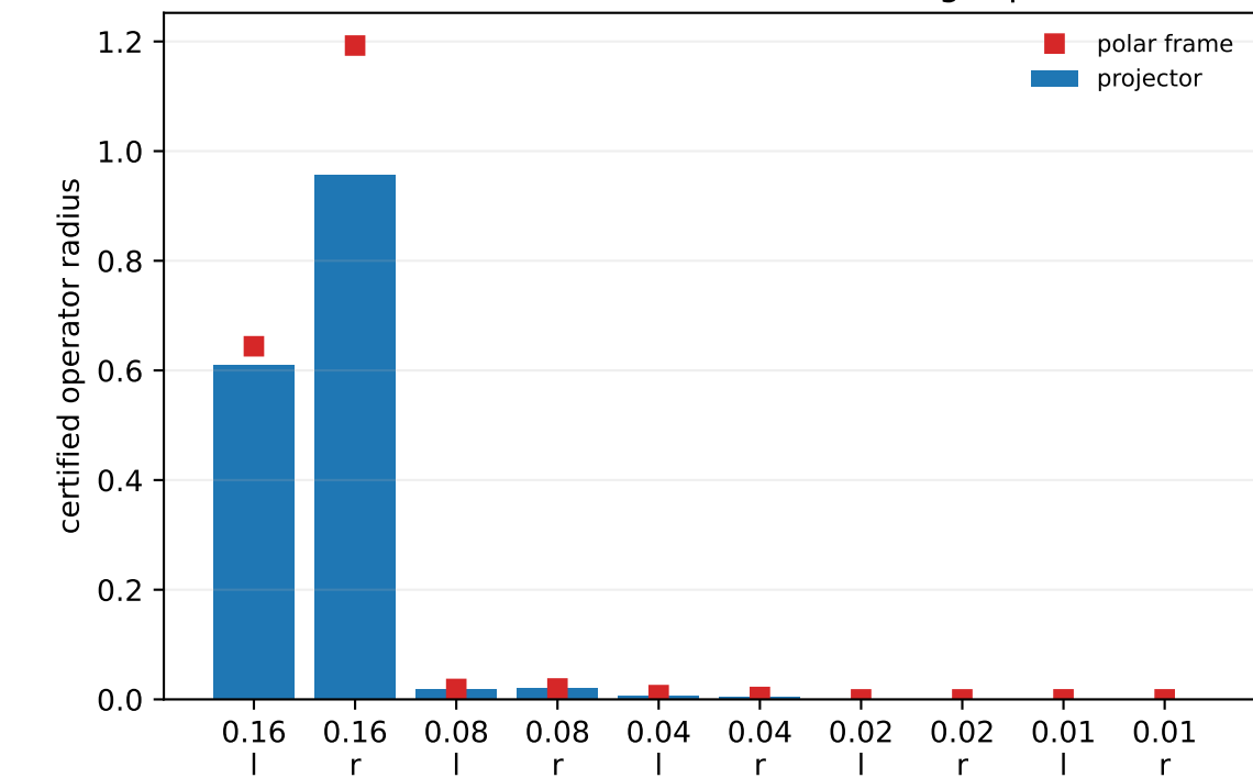
Certification is broad at the coarse right packet
