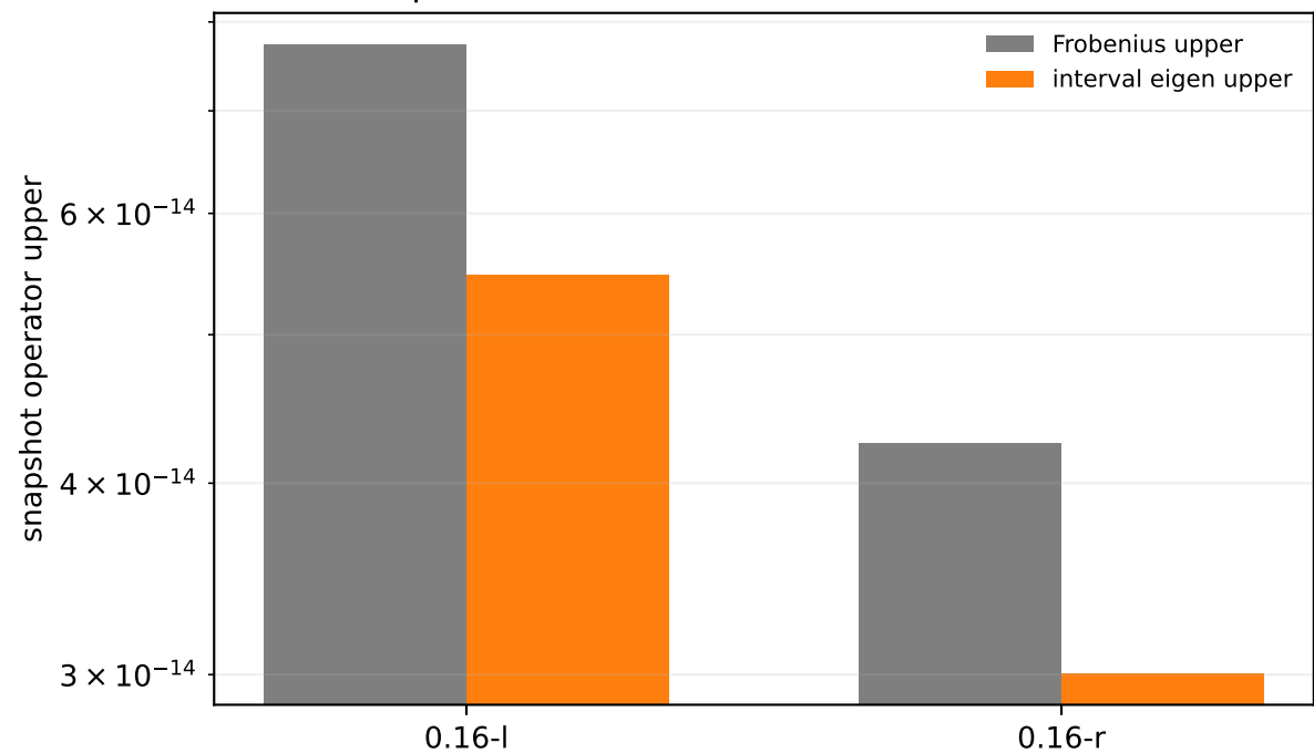
Sharp norm extraction crosses the two thin walls
