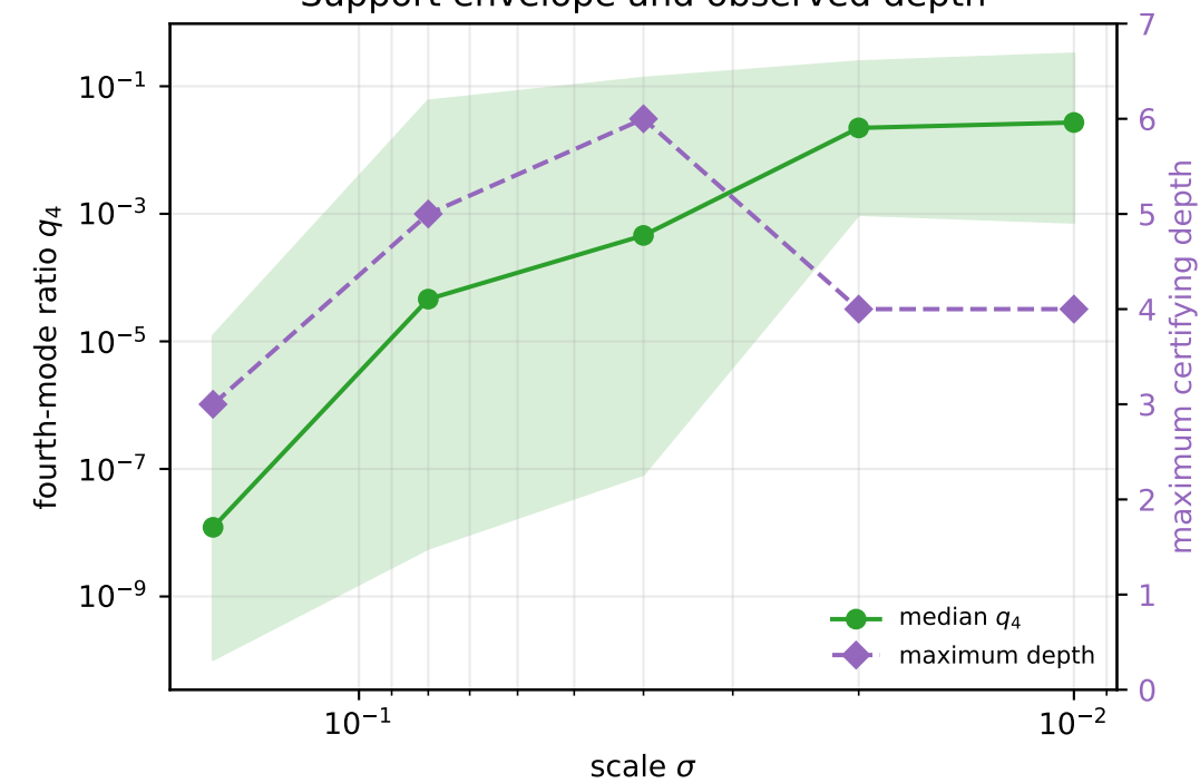
Support envelope and observed depth
