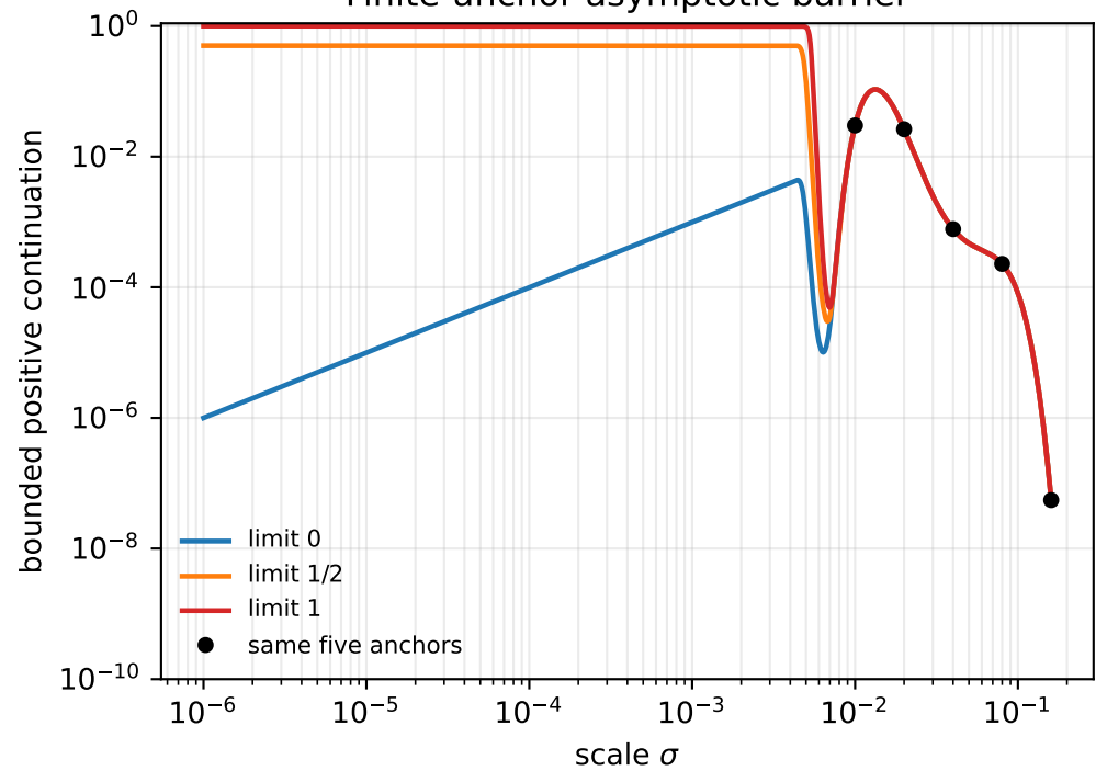
Finite-anchor asymptotic barrier
