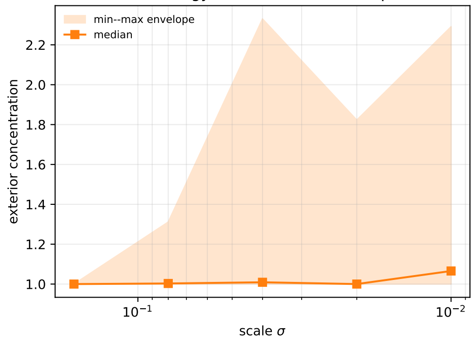
Tail-energy concentration envelope
