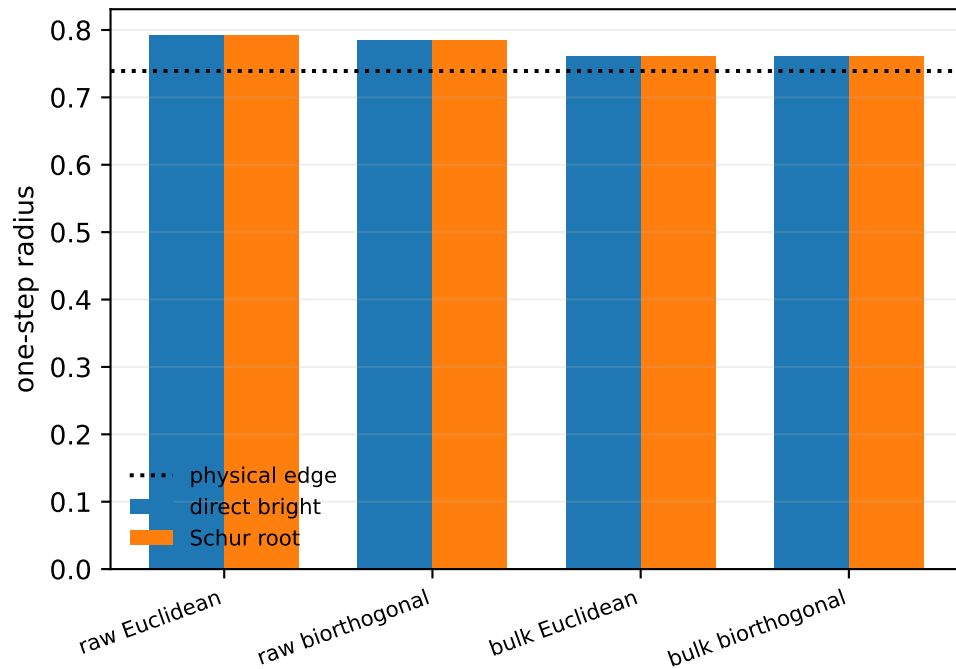
Peripheral extraction narrows but does not close the gap
