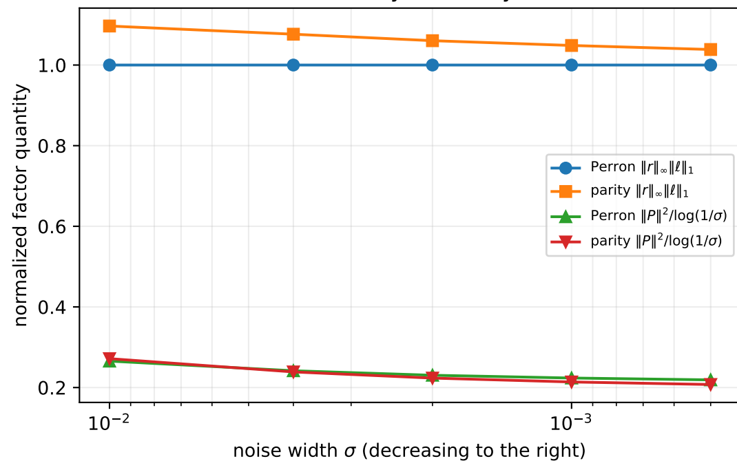
(a) Weak factors stay uniformly conditioned
