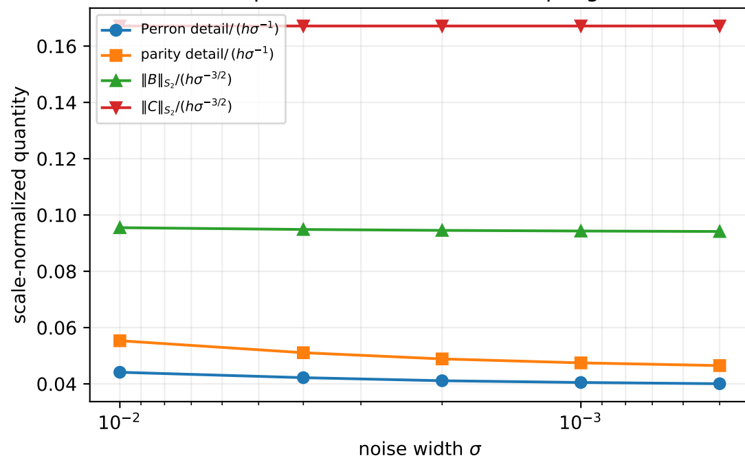
(b) Sharp detail and two-sided coupling clocks
