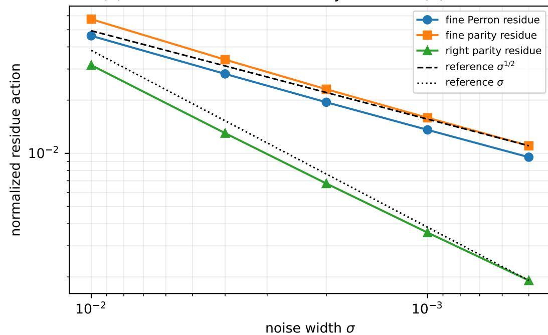
(c) Actual residues vanish beyond the O(1) theorem
