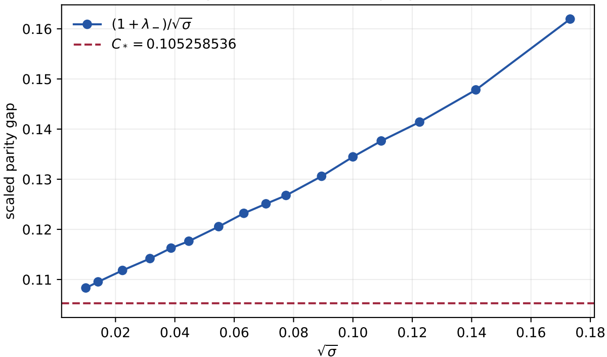
Convergence to the boundary-layer constant
